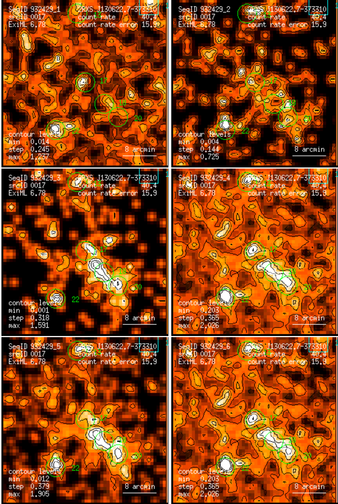
Figure 17: RASS 932429: detection 0017: band rate images, Gaussian filter: (1) PSPC channels 11 – 41, (2) 52 – 90, (3) 91 – 201, (4) 11 – 235, (5) 52 – 201, (6) 11 – 201. Broad band rates in counts/ks. Band rate contour levels in counts/ks/arcmin 2 .
