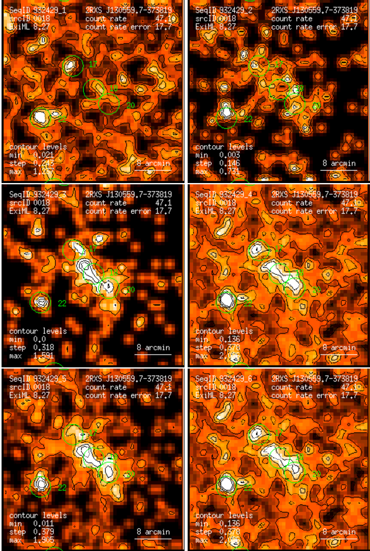
Figure 18: RASS 932429: detection 0018: band rate images, Gaussian filter: (1) PSPC channels 11 – 41, (2) 52 – 90, (3) 91 – 201, (4) 11 – 235, (5) 52 – 201, (6) 11 – 201. Broad band rates in counts/ks. Band rate contour levels in counts/ks/arcmin 2 .
