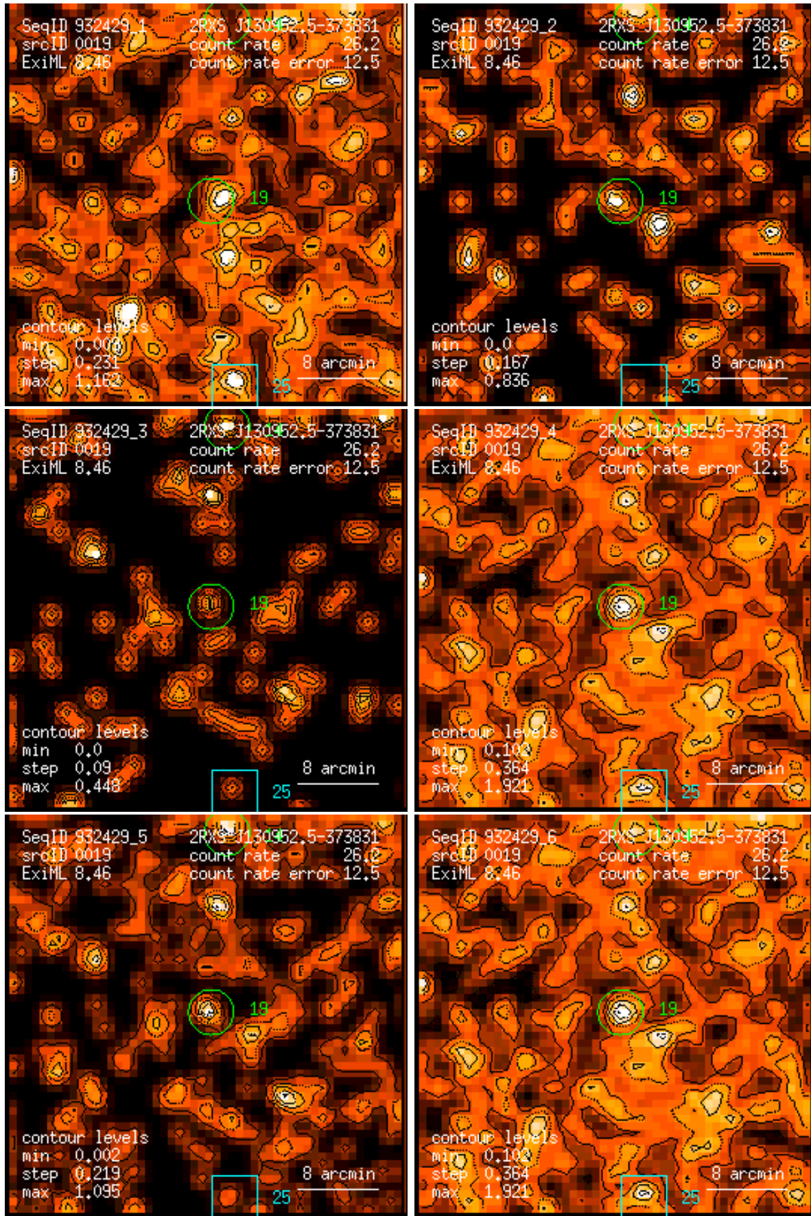
Figure 19: RASS 932429: detection 0019: band rate images, Gaussian filter: (1) PSPC channels 11 – 41, (2) 52 – 90, (3) 91 – 201, (4) 11 – 235, (5) 52 – 201, (6) 11 – 201. Broad band rates in counts/ks. Band rate contour levels in counts/ks/arcmin 2 .
