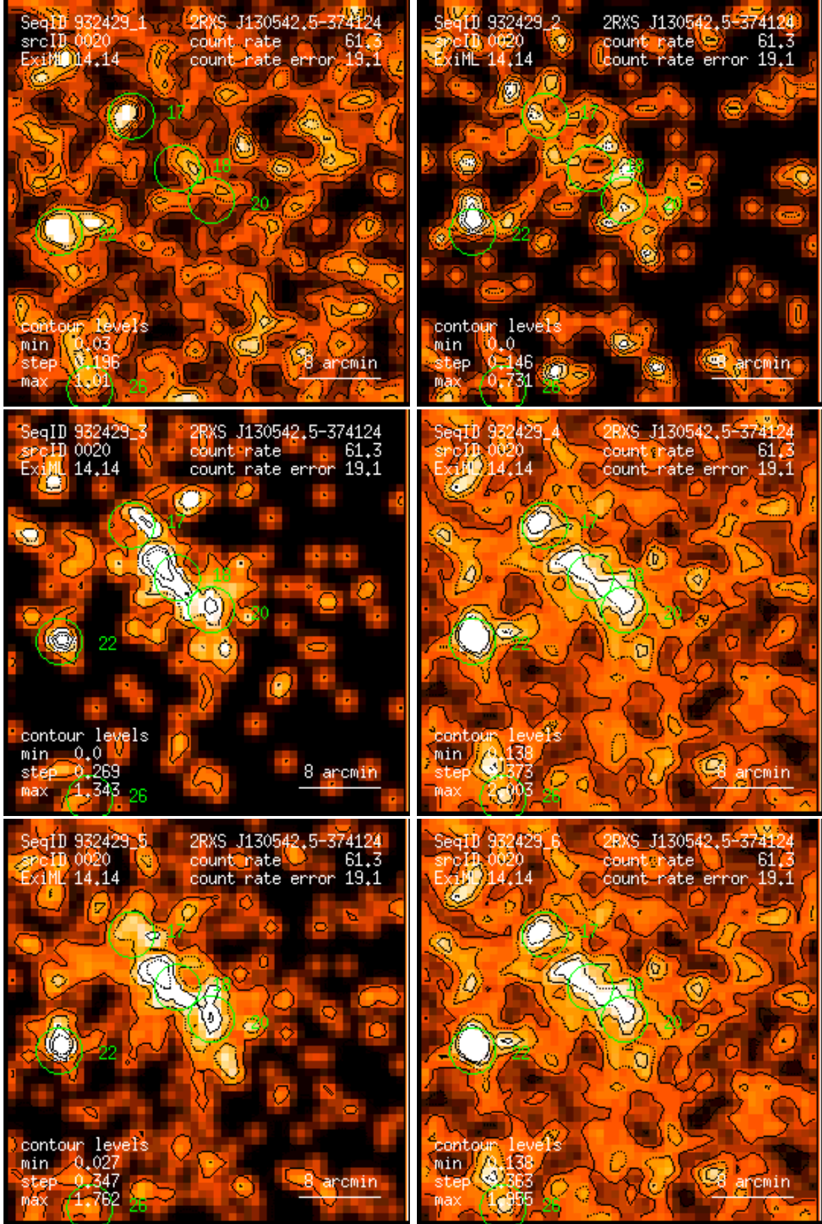
Figure 20: RASS 932429: detection 0020: band rate images, Gaussian filter: (1) PSPC channels 11 – 41, (2) 52 – 90, (3) 91 – 201, (4) 11 – 235, (5) 52 – 201, (6) 11 – 201. Broad band rates in counts/ks. Band rate contour levels in counts/ks/arcmin 2 .
