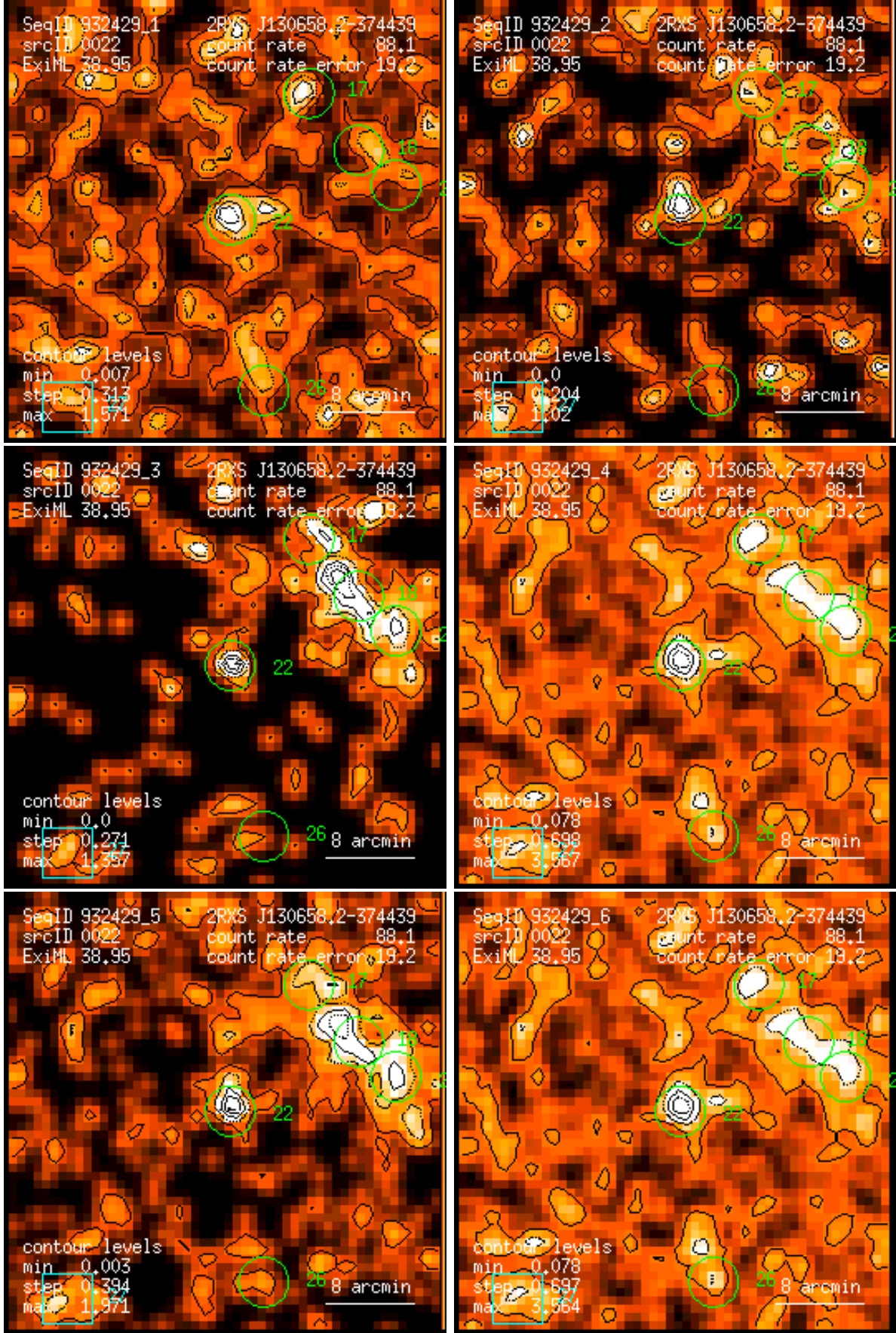
Figure 22: RASS 932429: detection 0022: band rate images, Gaussian filter: (1) PSPC channels 11 – 41, (2) 52 – 90, (3) 91 – 201, (4) 11 – 235, (5) 52 – 201, (6) 11 – 201. Broad band rates in counts/ks. Band rate contour levels in counts/ks/arcmin 2 .
