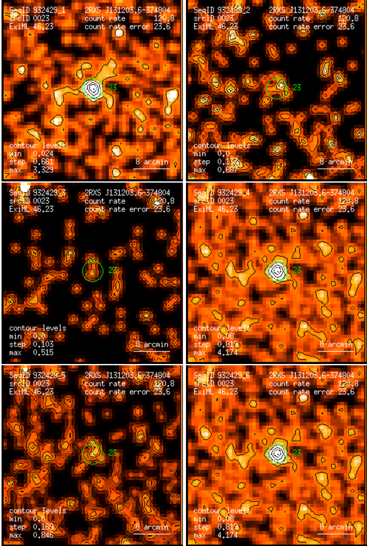
Figure 23: RASS 932429: detection 0023: band rate images, Gaussian filter: (1) PSPC channels 11 – 41, (2) 52 – 90, (3) 91 – 201, (4) 11 – 235, (5) 52 – 201, (6) 11 – 201. Broad band rates in counts/ks. Band rate contour levels in counts/ks/arcmin 2 .
