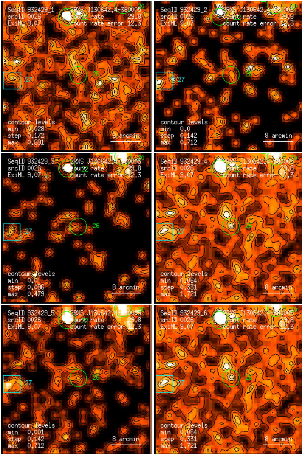
Figure 26: RASS 932429: detection 0026: band rate images, Gaussian filter: (1) PSPC channels 11 – 41, (2) 52 – 90, (3) 91 – 201, (4) 11 – 235, (5) 52 – 201, (6) 11 – 201. Broad band rates in counts/ks. Band rate contour levels in counts/ks/arcmin 2 .
