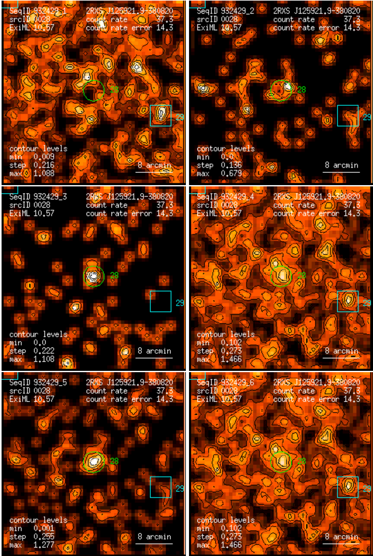
Figure 28: RASS 932429: detection 0028: band rate images, Gaussian filter: (1) PSPC channels 11 – 41, (2) 52 – 90, (3) 91 – 201, (4) 11 – 235, (5) 52 – 201, (6) 11 – 201. Broad band rates in counts/ks. Band rate contour levels in counts/ks/arcmin 2 .
