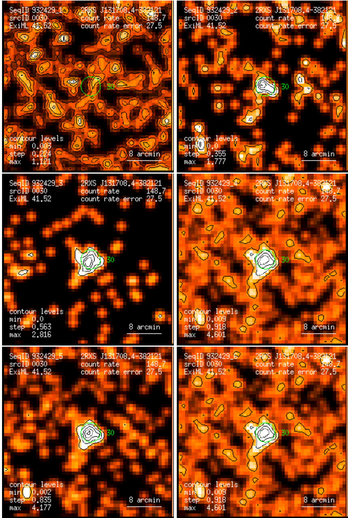
Figure 30: RASS 932429: detection 0030: band rate images, Gaussian filter: (1) PSPC channels 11 – 41, (2) 52 – 90, (3) 91 – 201, (4) 11 – 235, (5) 52 – 201, (6) 11 – 201. Broad band rates in counts/ks. Band rate contour levels in counts/ks/arcmin 2 .
