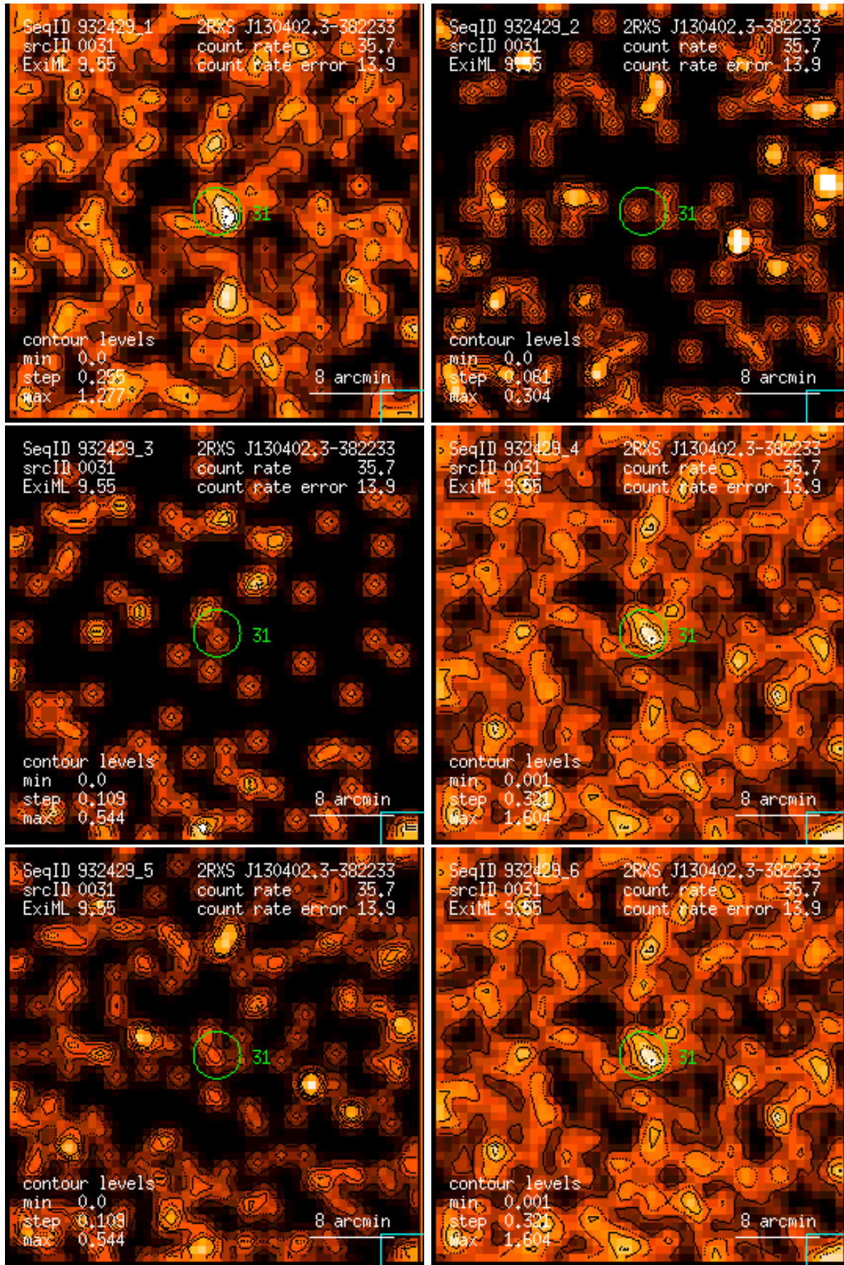
Figure 31: RASS 932429: detection 0031: band rate images, Gaussian filter: (1) PSPC channels 11 – 41, (2) 52 – 90, (3) 91 – 201, (4) 11 – 235, (5) 52 – 201, (6) 11 – 201. Broad band rates in counts/ks. Band rate contour levels in counts/ks/arcmin 2 .
