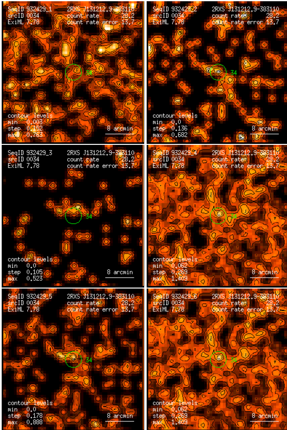
Figure 34: RASS 932429: detection 0034: band rate images, Gaussian filter: (1) PSPC channels 11 – 41, (2) 52 – 90, (3) 91 – 201, (4) 11 – 235, (5) 52 – 201, (6) 11 – 201. Broad band rates in counts/ks. Band rate contour levels in counts/ks/arcmin 2 .
