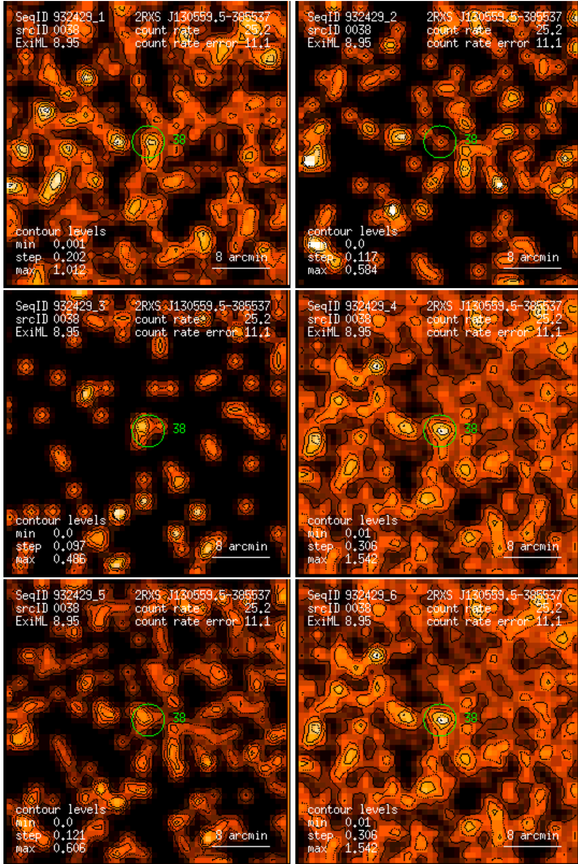
Figure 38: RASS 932429: detection 0038: band rate images, Gaussian filter: (1) PSPC channels 11 – 41, (2) 52 – 90, (3) 91 – 201, (4) 11 – 235, (5) 52 – 201, (6) 11 – 201. Broad band rates in counts/ks. Band rate contour levels in counts/ks/arcmin 2 .
