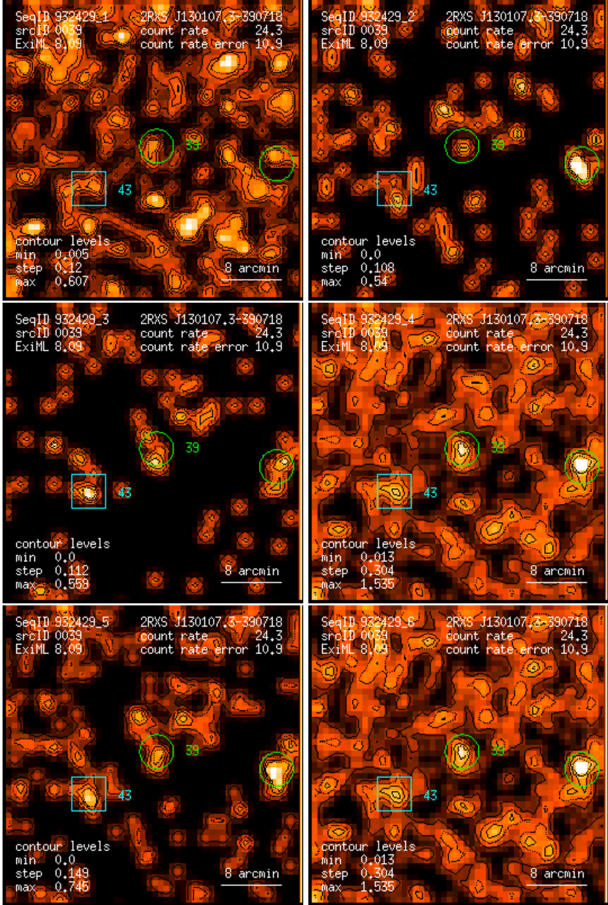
Figure 39: RASS 932429: detection 0039: band rate images, Gaussian filter: (1) PSPC channels 11 – 41, (2) 52 – 90, (3) 91 – 201, (4) 11 – 235, (5) 52 – 201, (6) 11 – 201. Broad band rates in counts/ks. Band rate contour levels in counts/ks/arcmin 2 .
