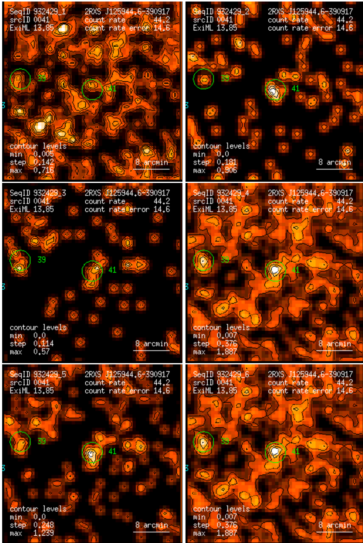
Figure 41: RASS 932429: detection 0041: band rate images, Gaussian filter: (1) PSPC channels 11 – 41, (2) 52 – 90, (3) 91 – 201, (4) 11 – 235, (5) 52 – 201, (6) 11 – 201. Broad band rates in counts/ks. Band rate contour levels in counts/ks/arcmin 2 .
