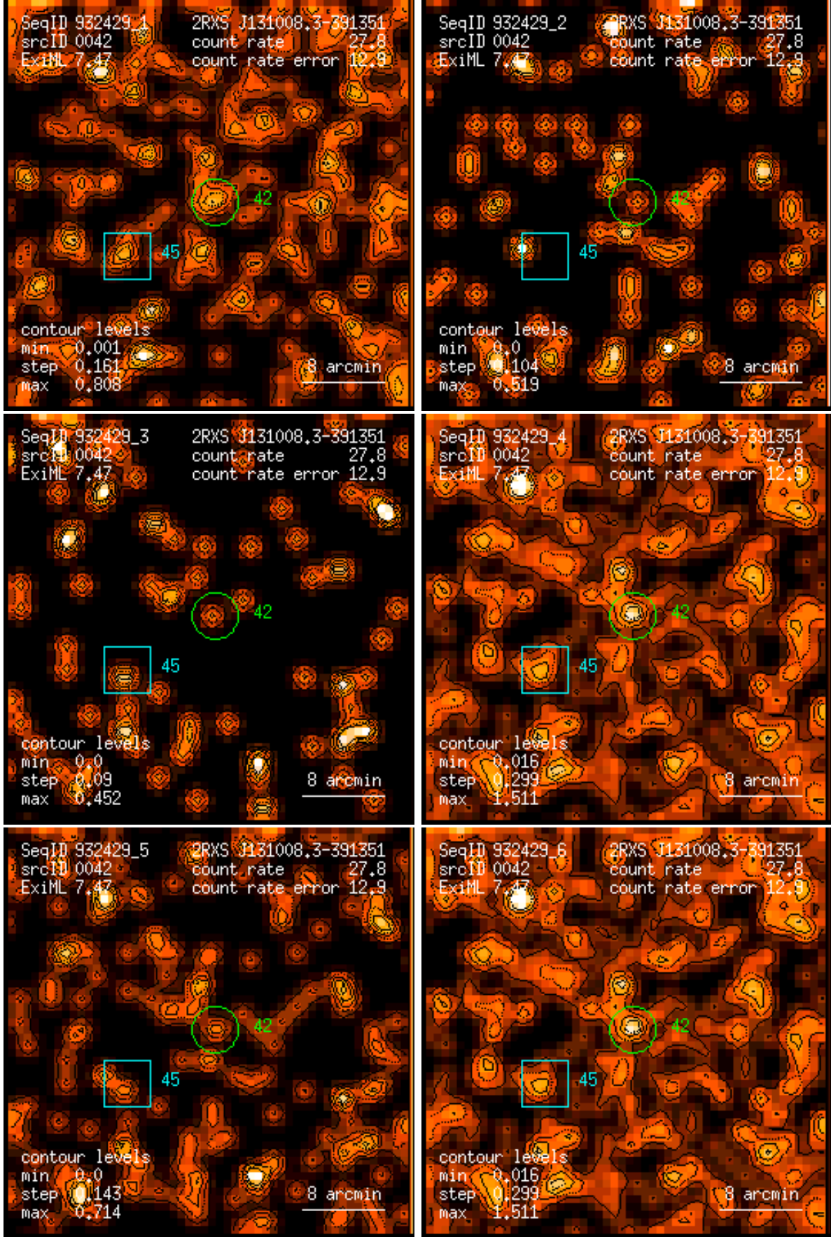
Figure 42: RASS 932429: detection 0042: band rate images, Gaussian filter: (1) PSPC channels 11 – 41, (2) 52 – 90, (3) 91 – 201, (4) 11 – 235, (5) 52 – 201, (6) 11 – 201. Broad band rates in counts/ks. Band rate contour levels in counts/ks/arcmin 2 .
