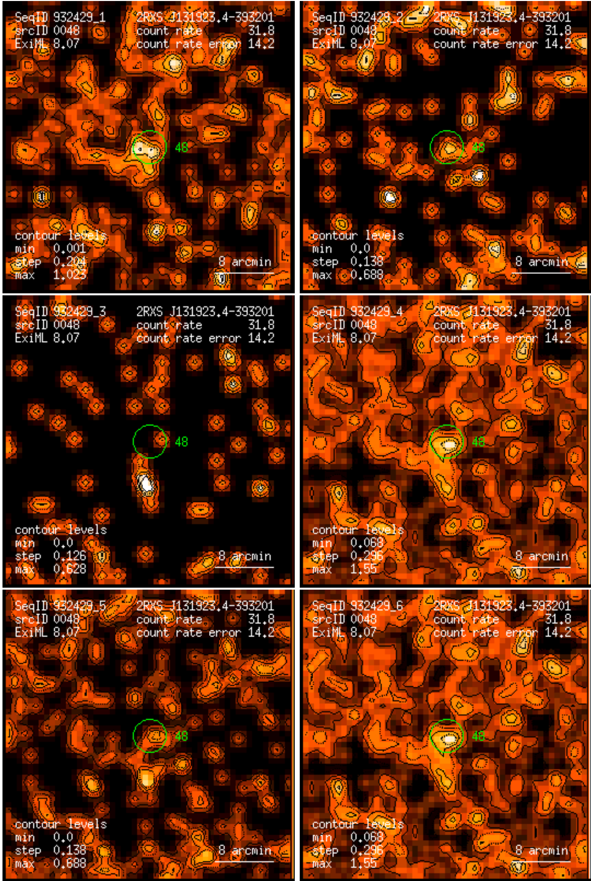
Figure 48: RASS 932429: detection 0048: band rate images, Gaussian filter: (1) PSPC channels 11 – 41, (2) 52 – 90, (3) 91 – 201, (4) 11 – 235, (5) 52 – 201, (6) 11 – 201. Broad band rates in counts/ks. Band rate contour levels in counts/ks/arcmin 2 .
