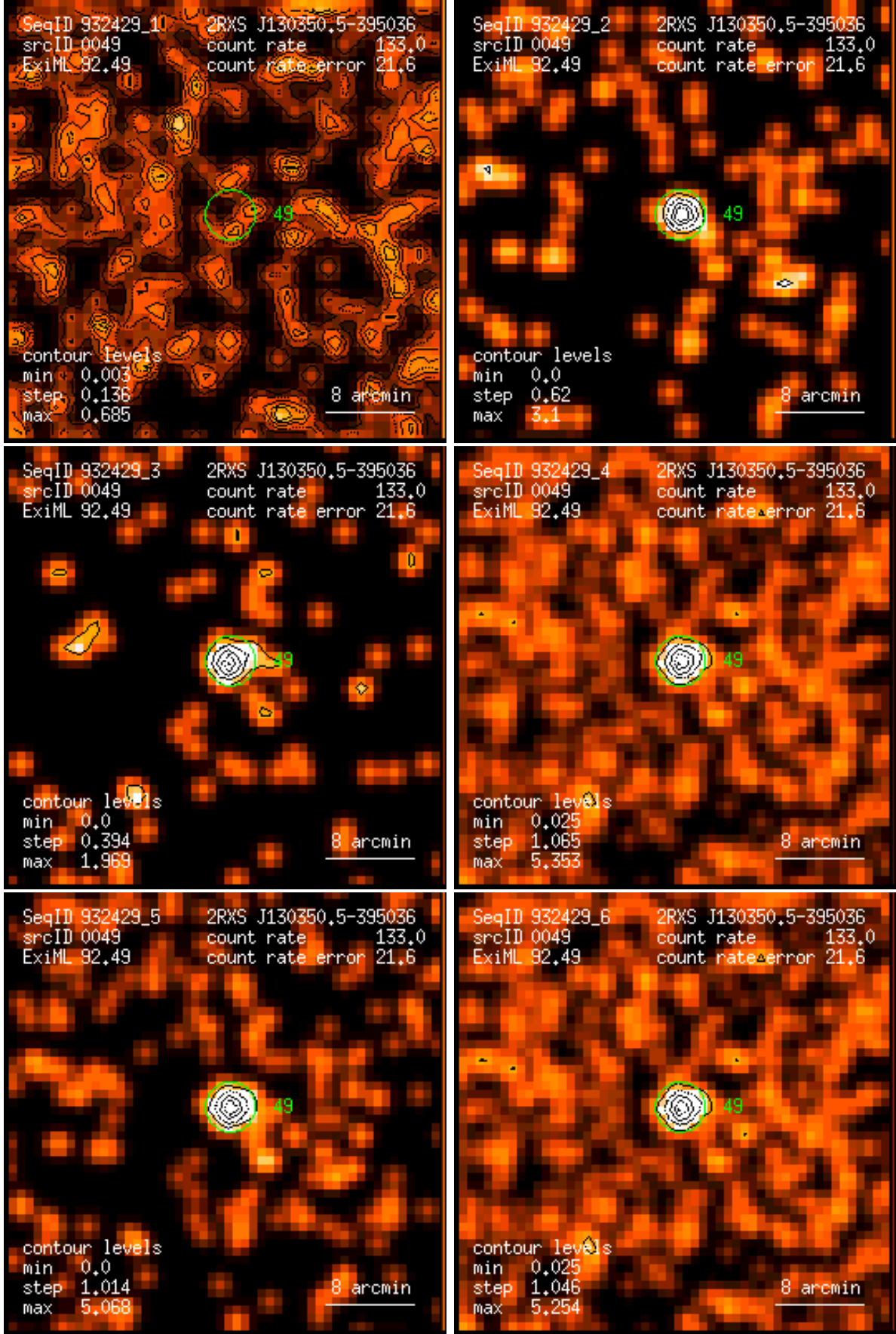
Figure 49: RASS 932429: detection 0049: band rate images, Gaussian filter: (1) PSPC channels 11 – 41, (2) 52 – 90, (3) 91 – 201, (4) 11 – 235, (5) 52 – 201, (6) 11 – 201. Broad band rates in counts/ks. Band rate contour levels in counts/ks/arcmin 2 .
