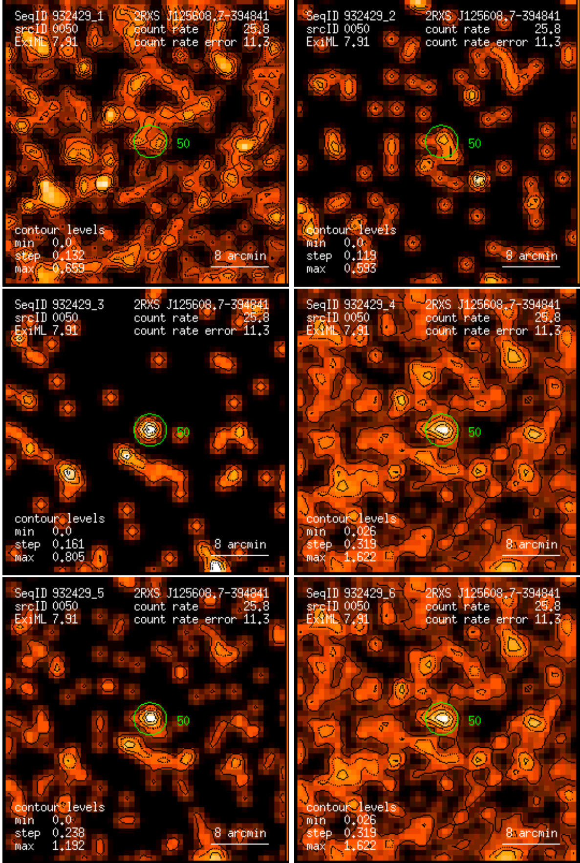
Figure 50: RASS 932429: detection 0050: band rate images, Gaussian filter: (1) PSPC channels 11 – 41, (2) 52 – 90, (3) 91 – 201, (4) 11 – 235, (5) 52 – 201, (6) 11 – 201. Broad band rates in counts/ks. Band rate contour levels in counts/ks/arcmin 2 .
