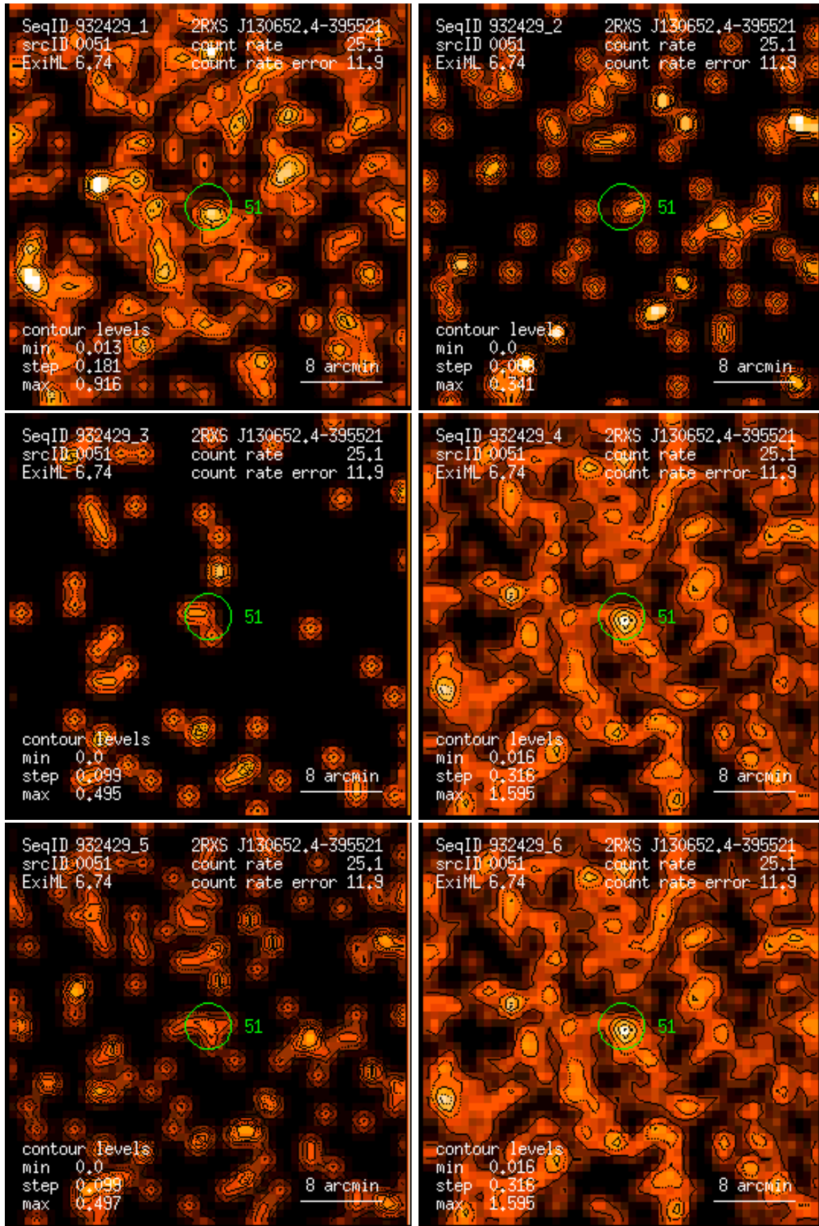
Figure 51: RASS 932429: detection 0051: band rate images, Gaussian filter: (1) PSPC channels 11 – 41, (2) 52 – 90, (3) 91 – 201, (4) 11 – 235, (5) 52 – 201, (6) 11 – 201. Broad band rates in counts/ks. Band rate contour levels in counts/ks/arcmin 2 .
