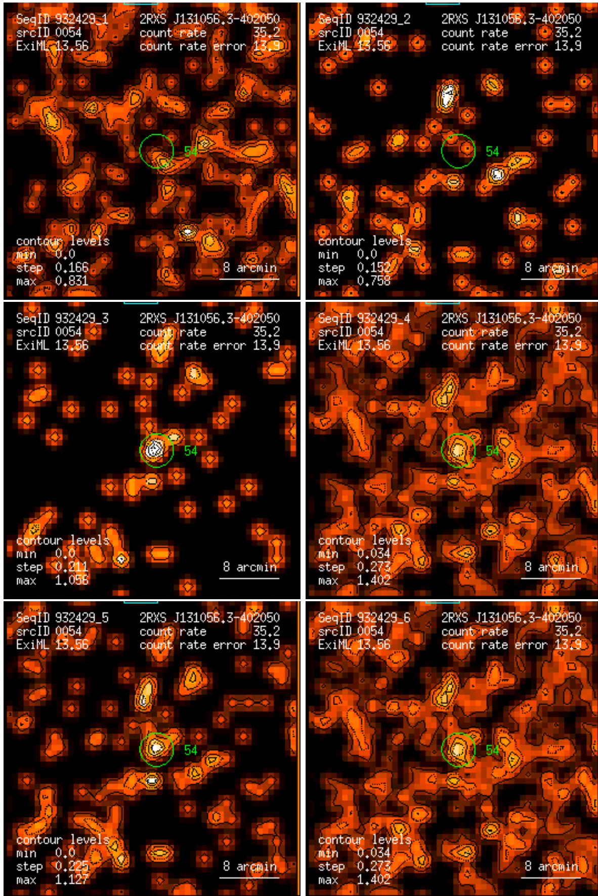
Figure 54: RASS 932429: detection 0054: band rate images, Gaussian filter: (1) PSPC channels 11 – 41, (2) 52 – 90, (3) 91 – 201, (4) 11 – 235, (5) 52 – 201, (6) 11 – 201. Broad band rates in counts/ks. Band rate contour levels in counts/ks/arcmin 2 .
