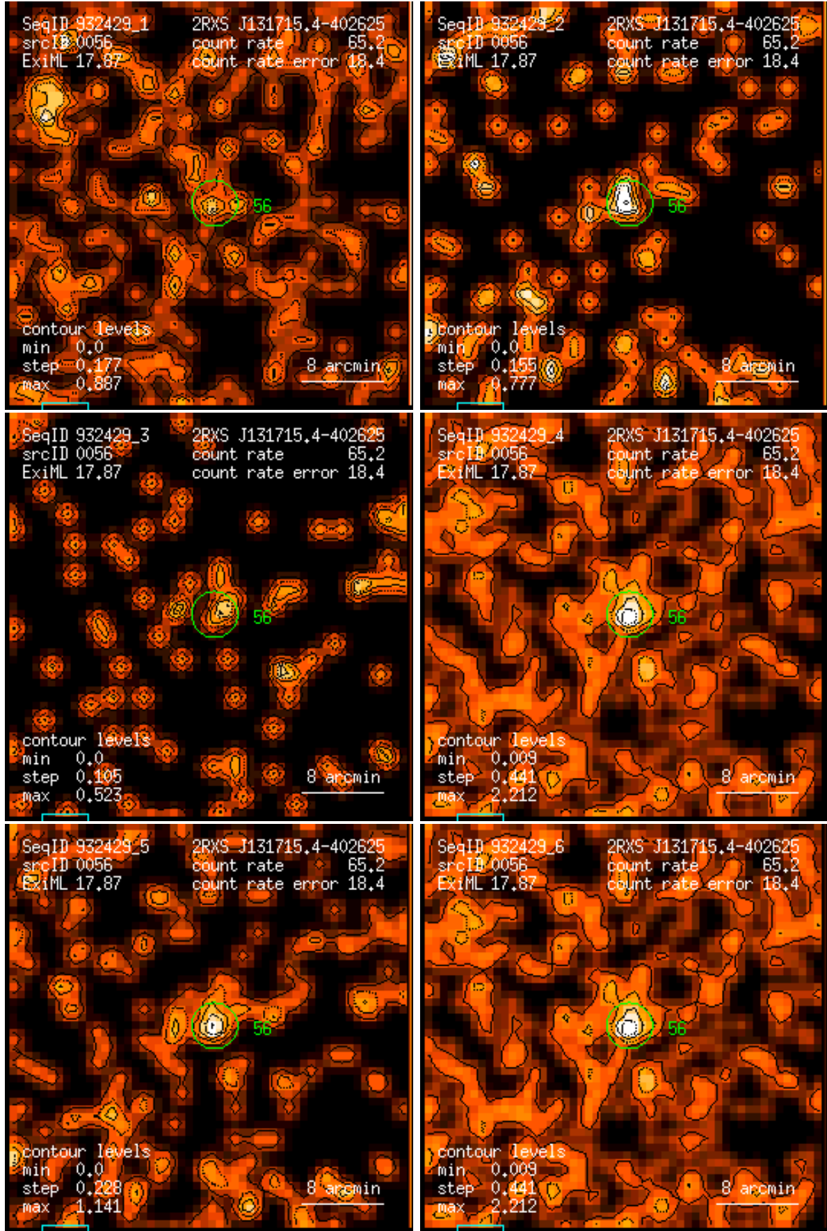
Figure 56: RASS 932429: detection 0056: band rate images, Gaussian filter: (1) PSPC channels 11 – 41, (2) 52 – 90, (3) 91 – 201, (4) 11 – 235, (5) 52 – 201, (6) 11 – 201. Broad band rates in counts/ks. Band rate contour levels in counts/ks/arcmin 2 .
