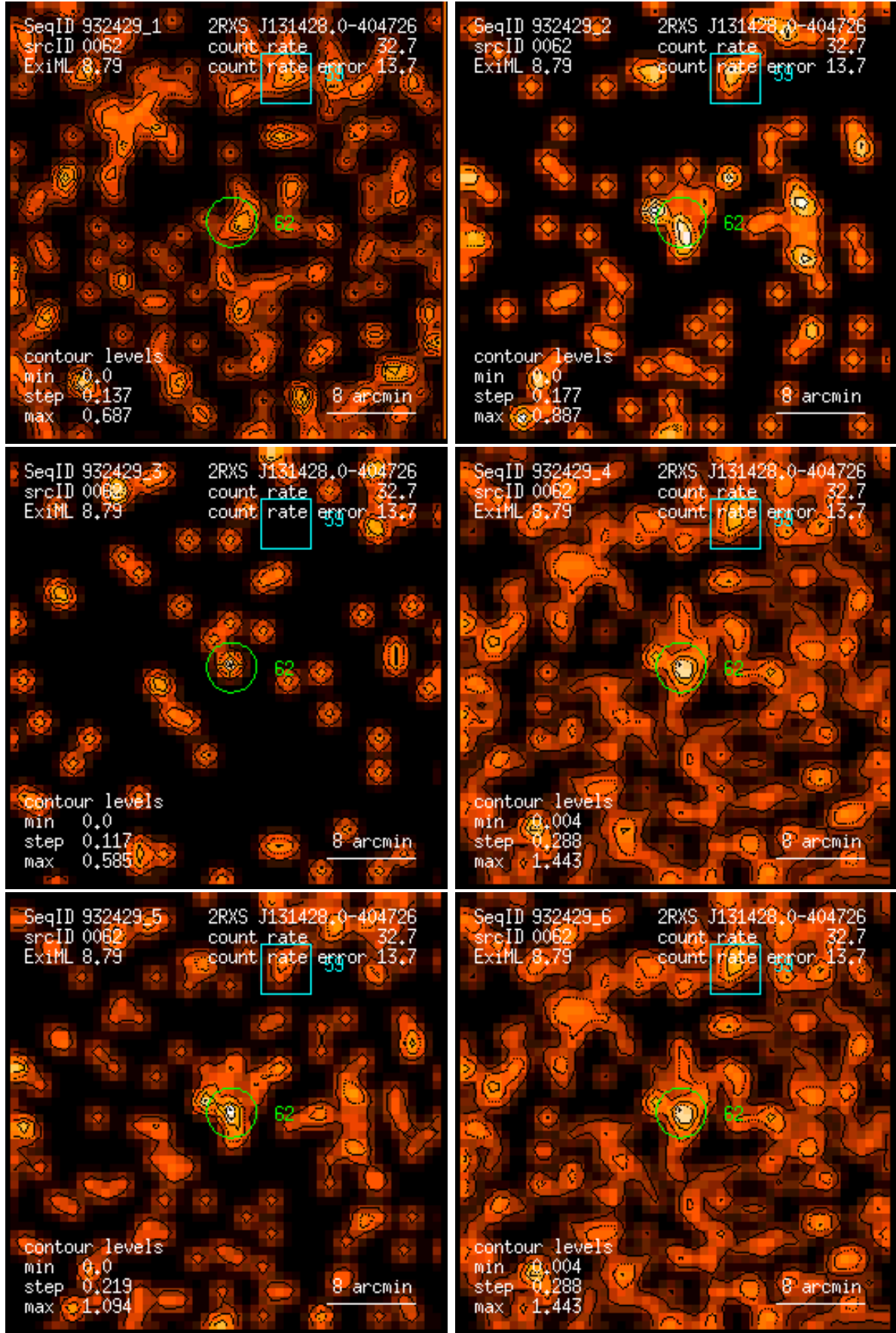
Figure 62: RASS 932429: detection 0062: band rate images, Gaussian filter: (1) PSPC channels 11 – 41, (2) 52 – 90, (3) 91 – 201, (4) 11 – 235, (5) 52 – 201, (6) 11 – 201. Broad band rates in counts/ks. Band rate contour levels in counts/ks/arcmin 2 .
