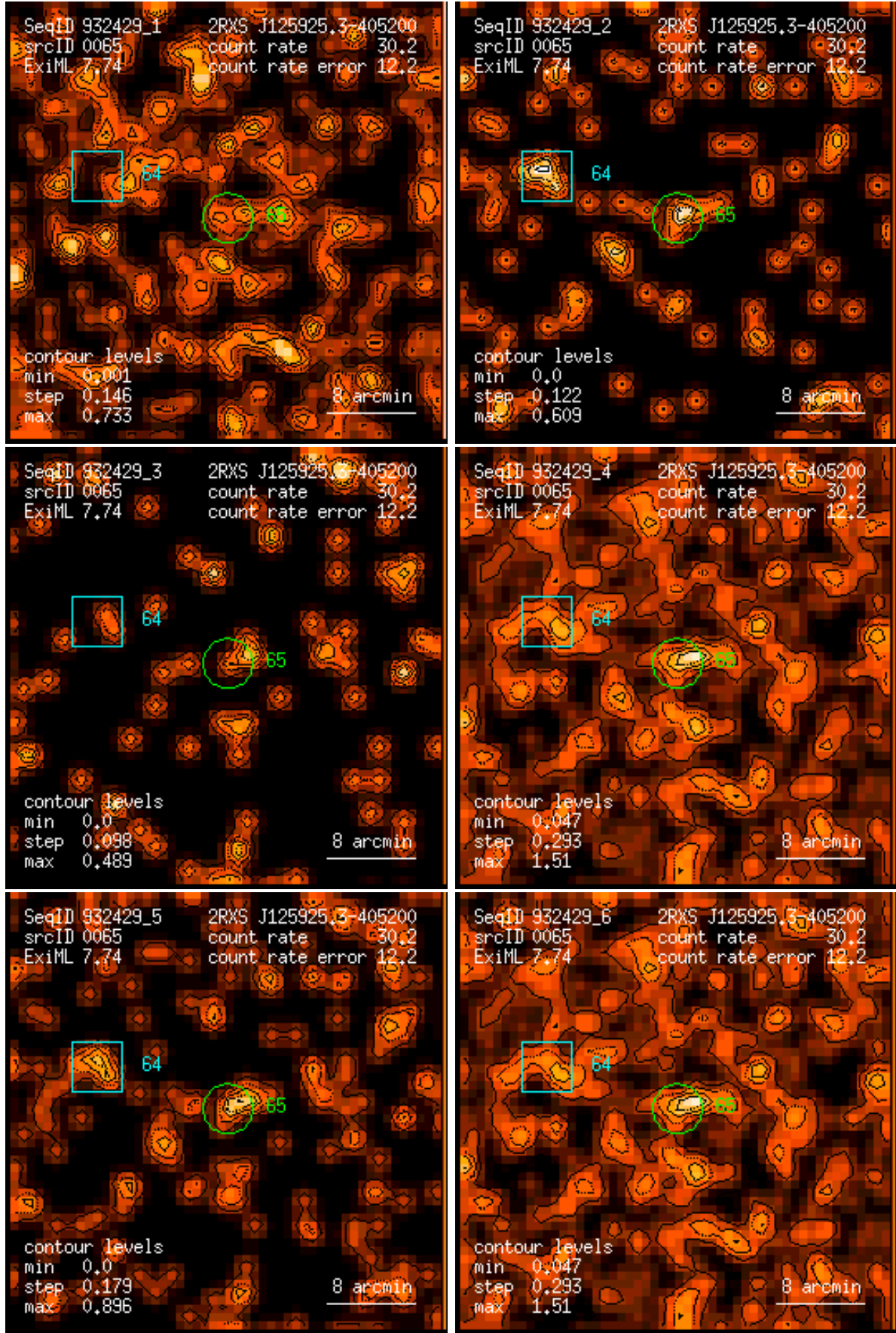
Figure 65: RASS 932429: detection 0065: band rate images, Gaussian filter: (1) PSPC channels 11 – 41, (2) 52 – 90, (3) 91 – 201, (4) 11 – 235, (5) 52 – 201, (6) 11 – 201. Broad band rates in counts/ks. Band rate contour levels in counts/ks/arcmin 2 .
