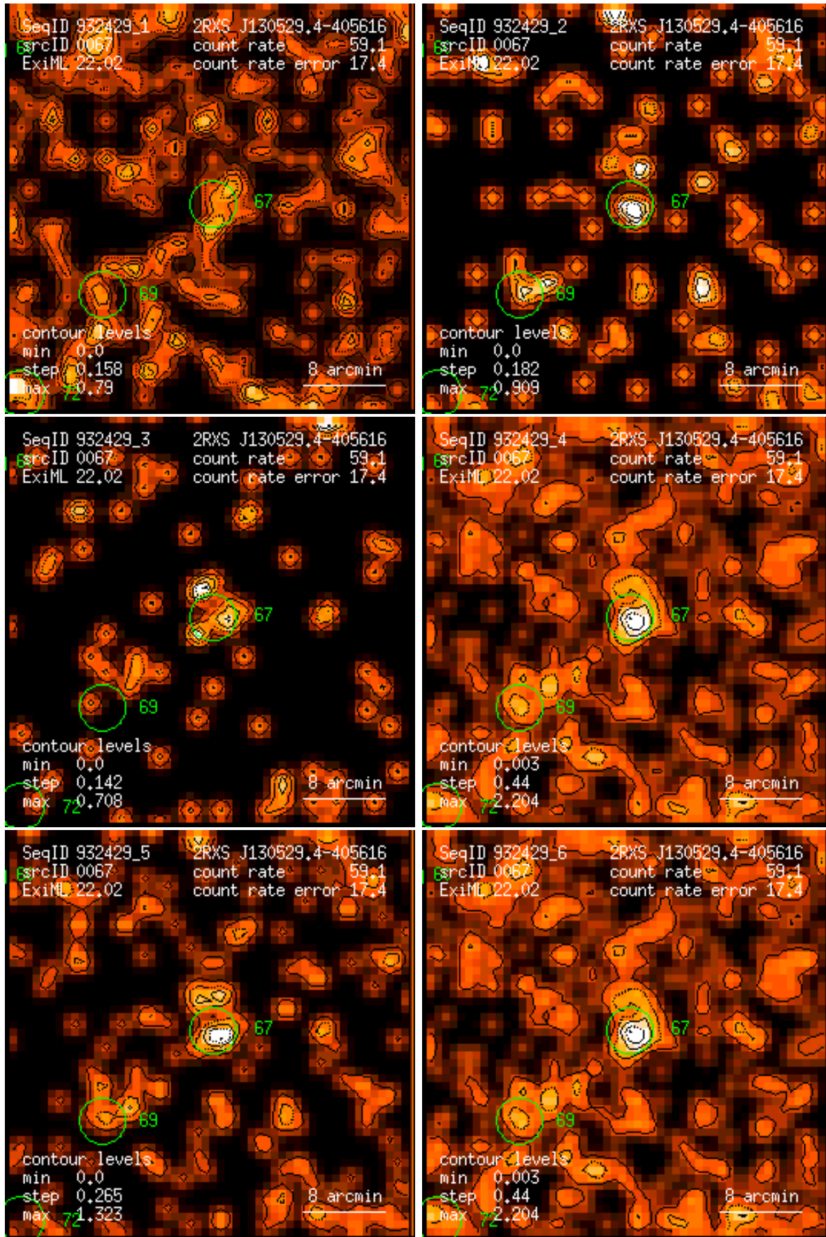
Figure 67: RASS 932429: detection 0067: band rate images, Gaussian filter: (1) PSPC channels 11 – 41, (2) 52 – 90, (3) 91 – 201, (4) 11 – 235, (5) 52 – 201, (6) 11 – 201. Broad band rates in counts/ks. Band rate contour levels in counts/ks/arcmin 2 .
