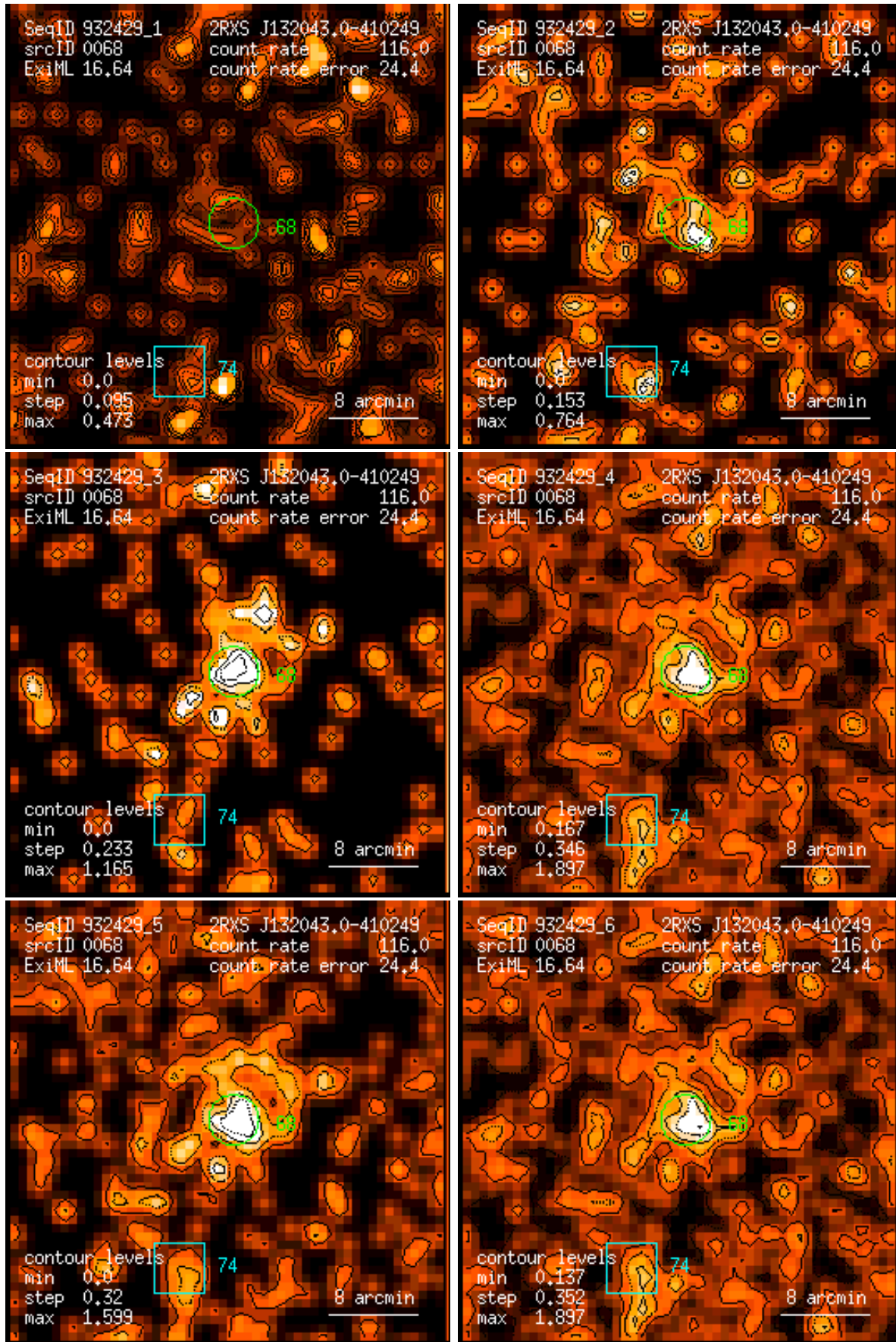
Figure 68: RASS 932429: detection 0068: band rate images, Gaussian filter: (1) PSPC channels 11 – 41, (2) 52 – 90, (3) 91 – 201, (4) 11 – 235, (5) 52 – 201, (6) 11 – 201. Broad band rates in counts/ks. Band rate contour levels in counts/ks/arcmin 2 .
