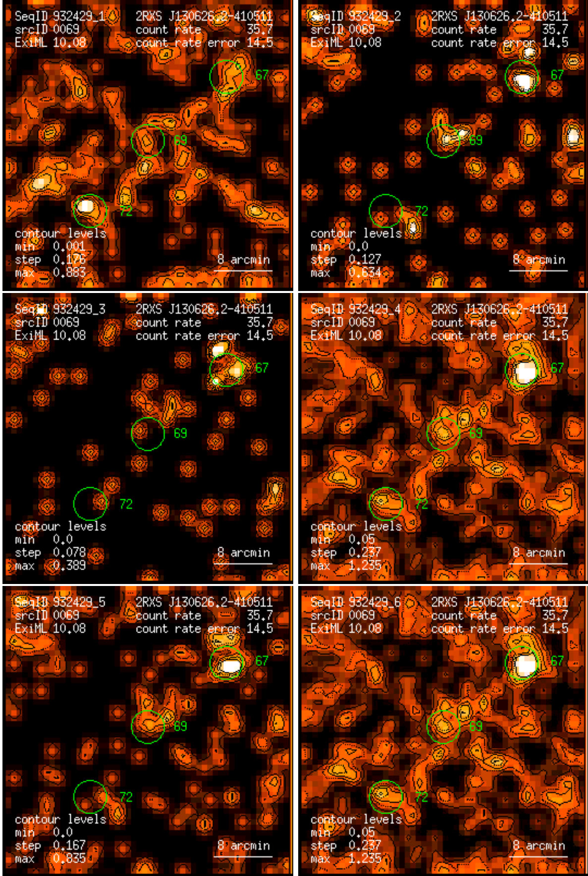
Figure 69: RASS 932429: detection 0069: band rate images, Gaussian filter: (1) PSPC channels 11 – 41, (2) 52 – 90, (3) 91 – 201, (4) 11 – 235, (5) 52 – 201, (6) 11 – 201. Broad band rates in counts/ks. Band rate contour levels in counts/ks/arcmin 2 .
