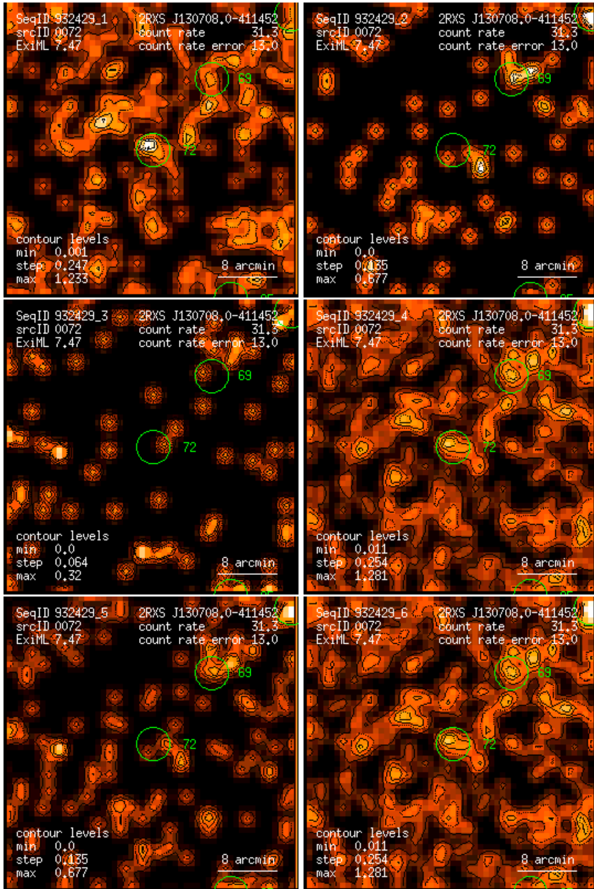
Figure 72: RASS 932429: detection 0072: band rate images, Gaussian filter: (1) PSPC channels 11 – 41, (2) 52 – 90, (3) 91 – 201, (4) 11 – 235, (5) 52 – 201, (6) 11 – 201. Broad band rates in counts/ks. Band rate contour levels in counts/ks/arcmin 2 .
