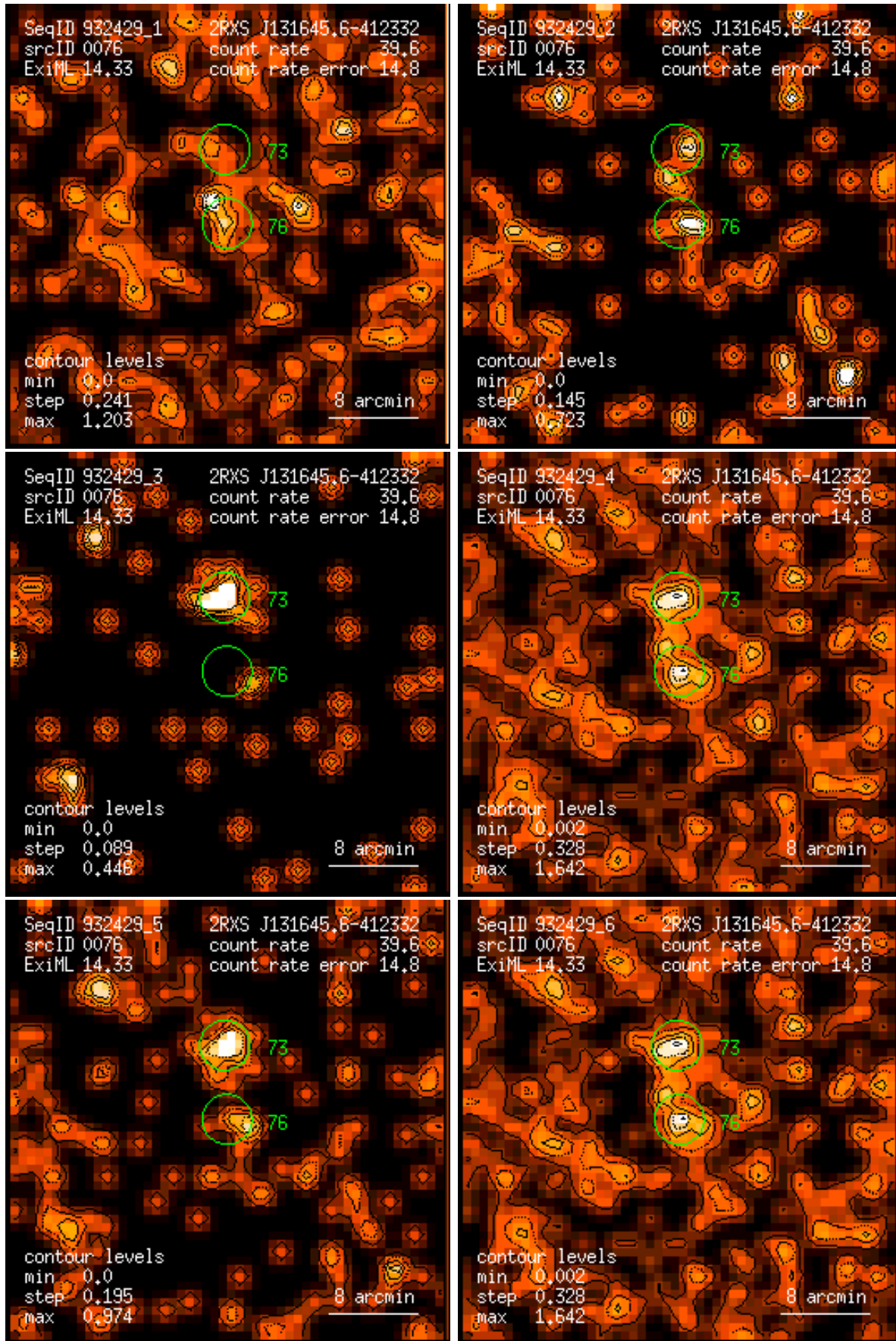
Figure 76: RASS 932429: detection 0076: band rate images, Gaussian filter: (1) PSPC channels 11 – 41, (2) 52 – 90, (3) 91 – 201, (4) 11 – 235, (5) 52 – 201, (6) 11 – 201. Broad band rates in counts/ks. Band rate contour levels in counts/ks/arcmin 2 .
