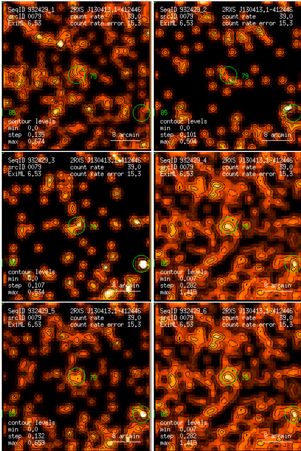
Figure 79: RASS 932429: detection 0079: band rate images, Gaussian filter: (1) PSPC channels 11 – 41, (2) 52 – 90, (3) 91 – 201, (4) 11 – 235, (5) 52 – 201, (6) 11 – 201. Broad band rates in counts/ks. Band rate contour levels in counts/ks/arcmin 2 .
