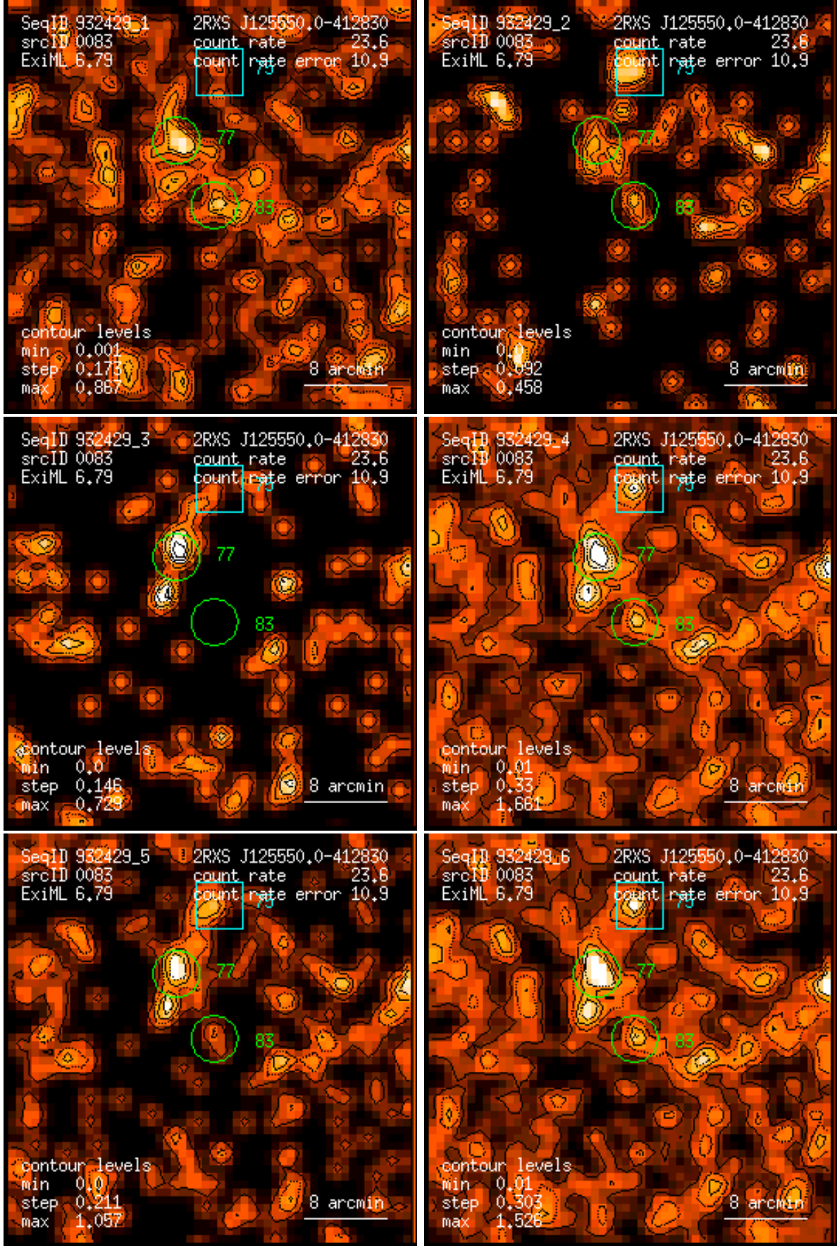
Figure 83: RASS 932429: detection 0083: band rate images, Gaussian filter: (1) PSPC channels 11 – 41, (2) 52 – 90, (3) 91 – 201, (4) 11 – 235, (5) 52 – 201, (6) 11 – 201. Broad band rates in counts/ks. Band rate contour levels in counts/ks/arcmin 2 .
