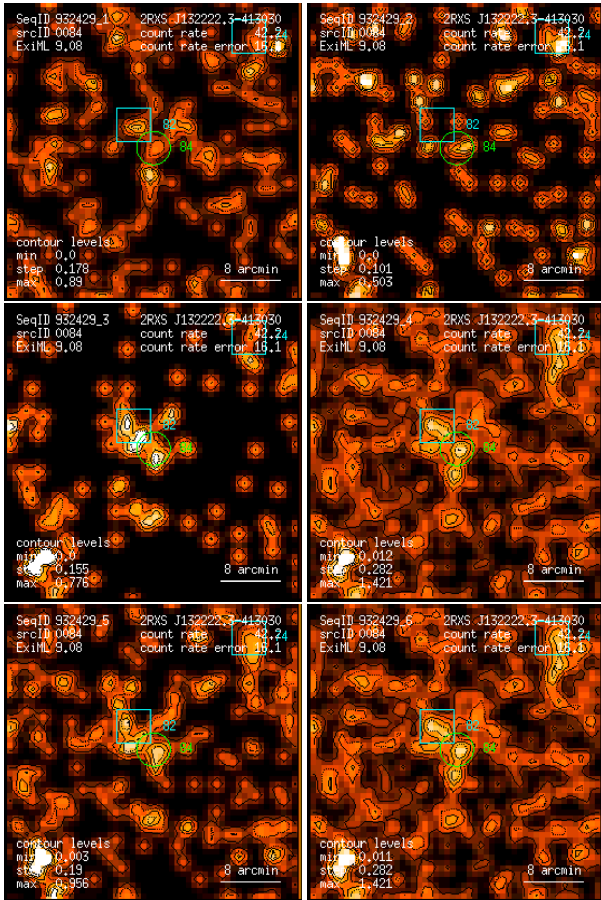
Figure 84: RASS 932429: detection 0084: band rate images, Gaussian filter: (1) PSPC channels 11 – 41, (2) 52 – 90, (3) 91 – 201, (4) 11 – 235, (5) 52 – 201, (6) 11 – 201. Broad band rates in counts/ks. Band rate contour levels in counts/ks/arcmin 2 .
