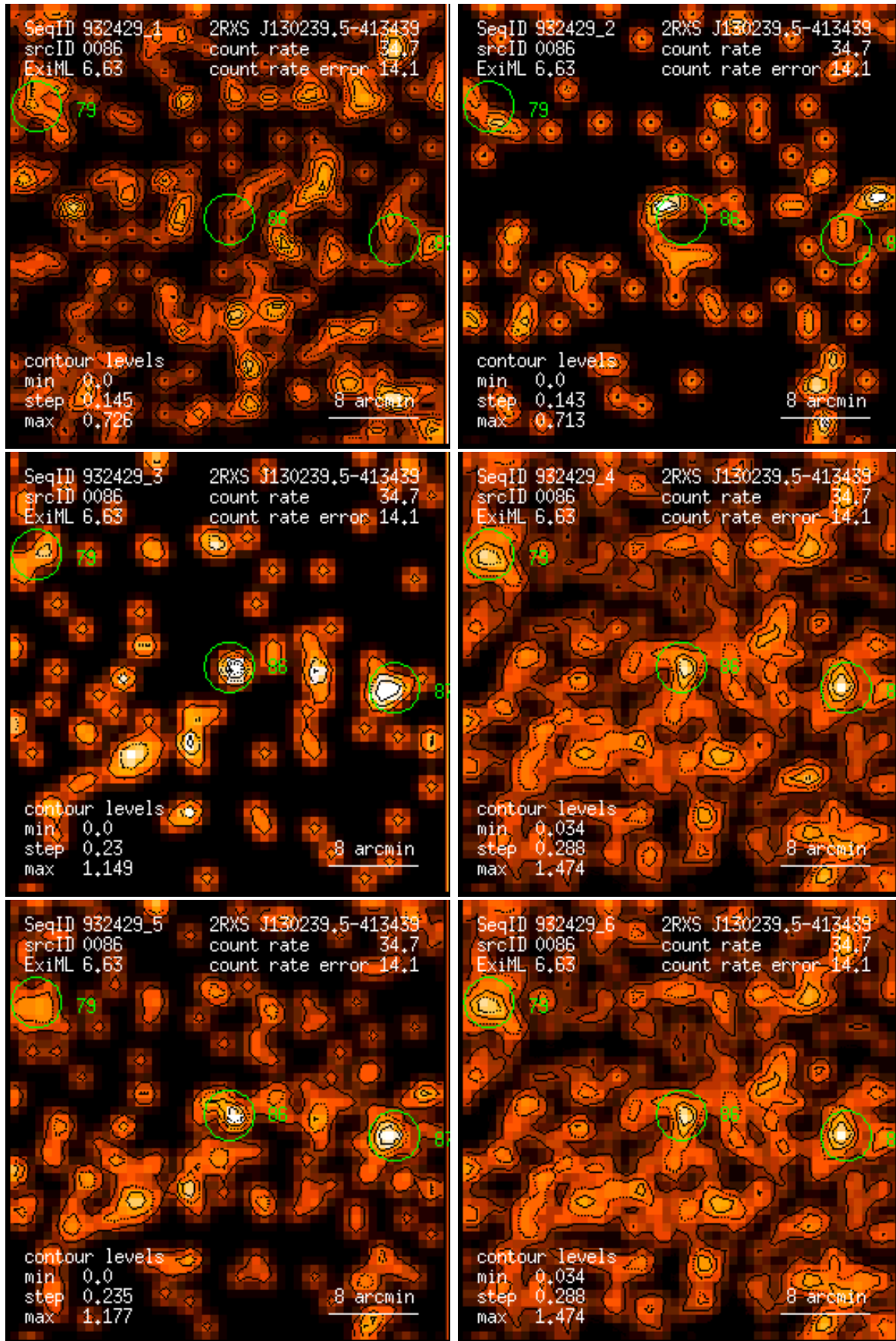
Figure 86: RASS 932429: detection 0086: band rate images, Gaussian filter: (1) PSPC channels 11 – 41, (2) 52 – 90, (3) 91 – 201, (4) 11 – 235, (5) 52 – 201, (6) 11 – 201. Broad band rates in counts/ks. Band rate contour levels in counts/ks/arcmin 2 .
