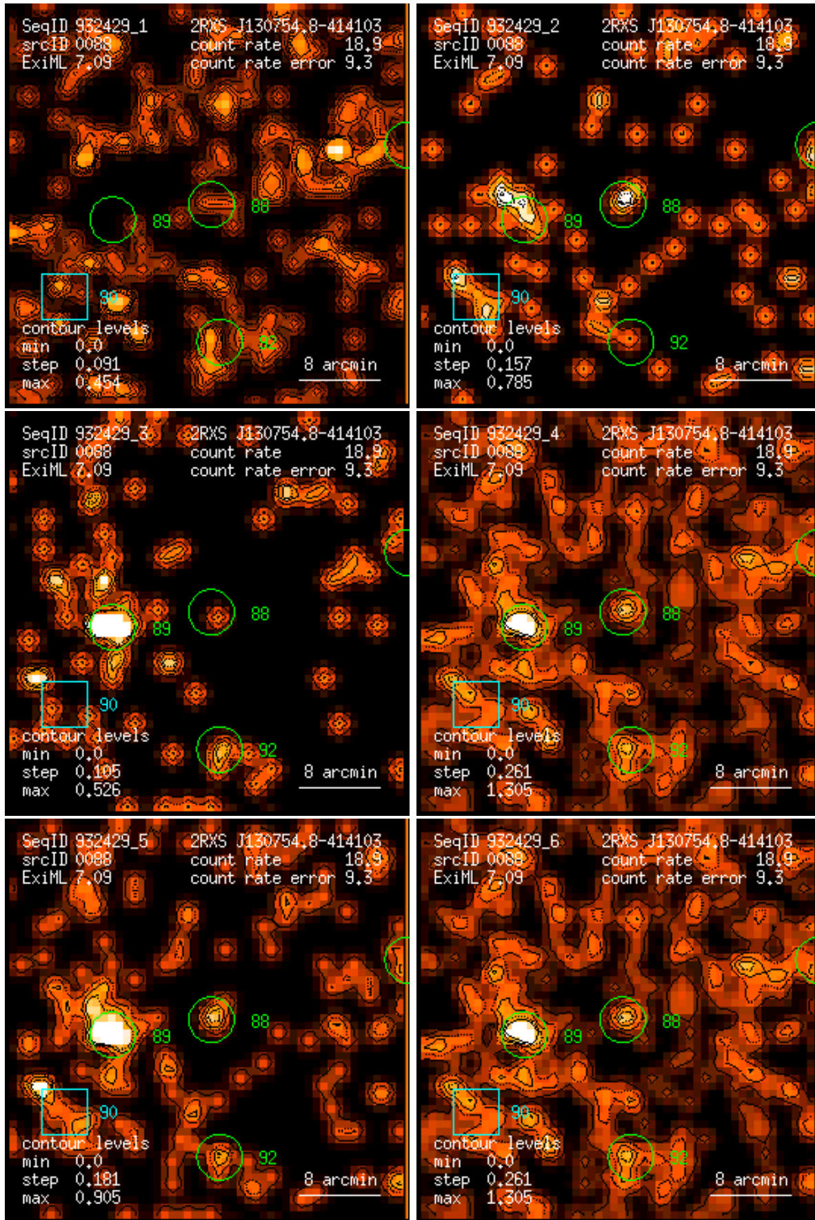
Figure 88: RASS 932429: detection 0088: band rate images, Gaussian filter: (1) PSPC channels 11 – 41, (2) 52 – 90, (3) 91 – 201, (4) 11 – 235, (5) 52 – 201, (6) 11 – 201. Broad band rates in counts/ks. Band rate contour levels in counts/ks/arcmin 2 .
