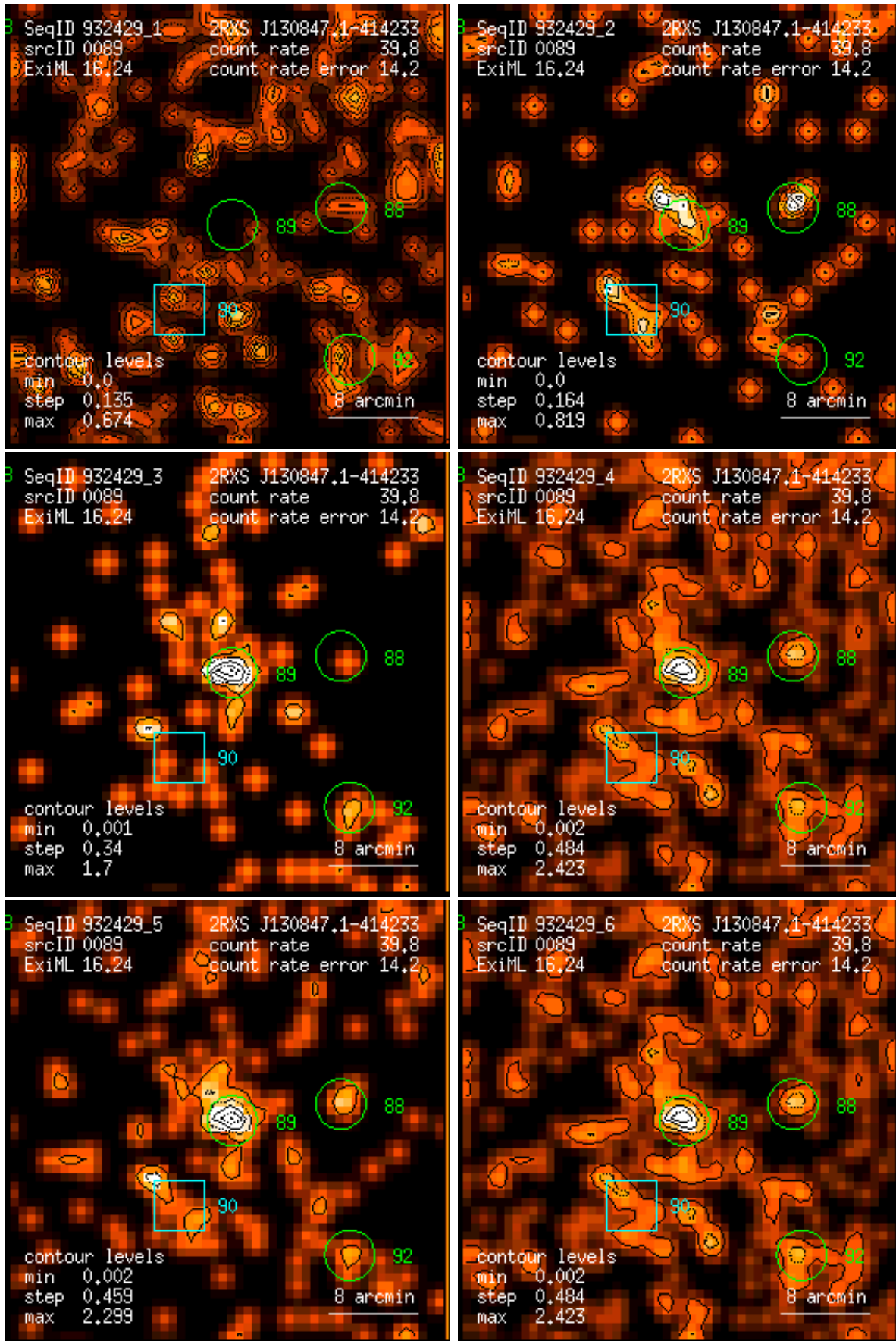
Figure 89: RASS 932429: detection 0089: band rate images, Gaussian filter: (1) PSPC channels 11 – 41, (2) 52 – 90, (3) 91 – 201, (4) 11 – 235, (5) 52 – 201, (6) 11 – 201. Broad band rates in counts/ks. Band rate contour levels in counts/ks/arcmin 2 .
