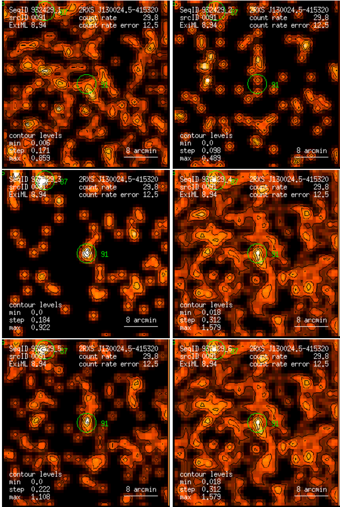
Figure 91: RASS 932429: detection 0091: band rate images, Gaussian filter: (1) PSPC channels 11 – 41, (2) 52 – 90, (3) 91 – 201, (4) 11 – 235, (5) 52 – 201, (6) 11 – 201. Broad band rates in counts/ks. Band rate contour levels in counts/ks/arcmin 2 .
