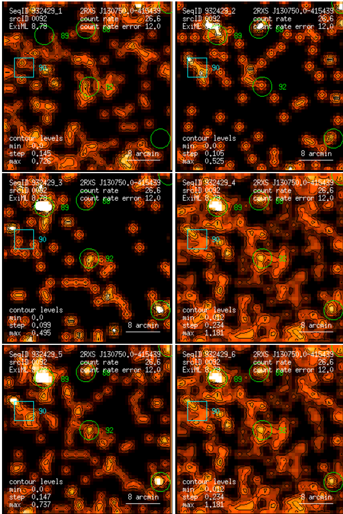
Figure 92: RASS 932429: detection 0092: band rate images, Gaussian filter: (1) PSPC channels 11 – 41, (2) 52 – 90, (3) 91 – 201, (4) 11 – 235, (5) 52 – 201, (6) 11 – 201. Broad band rates in counts/ks. Band rate contour levels in counts/ks/arcmin 2 .
