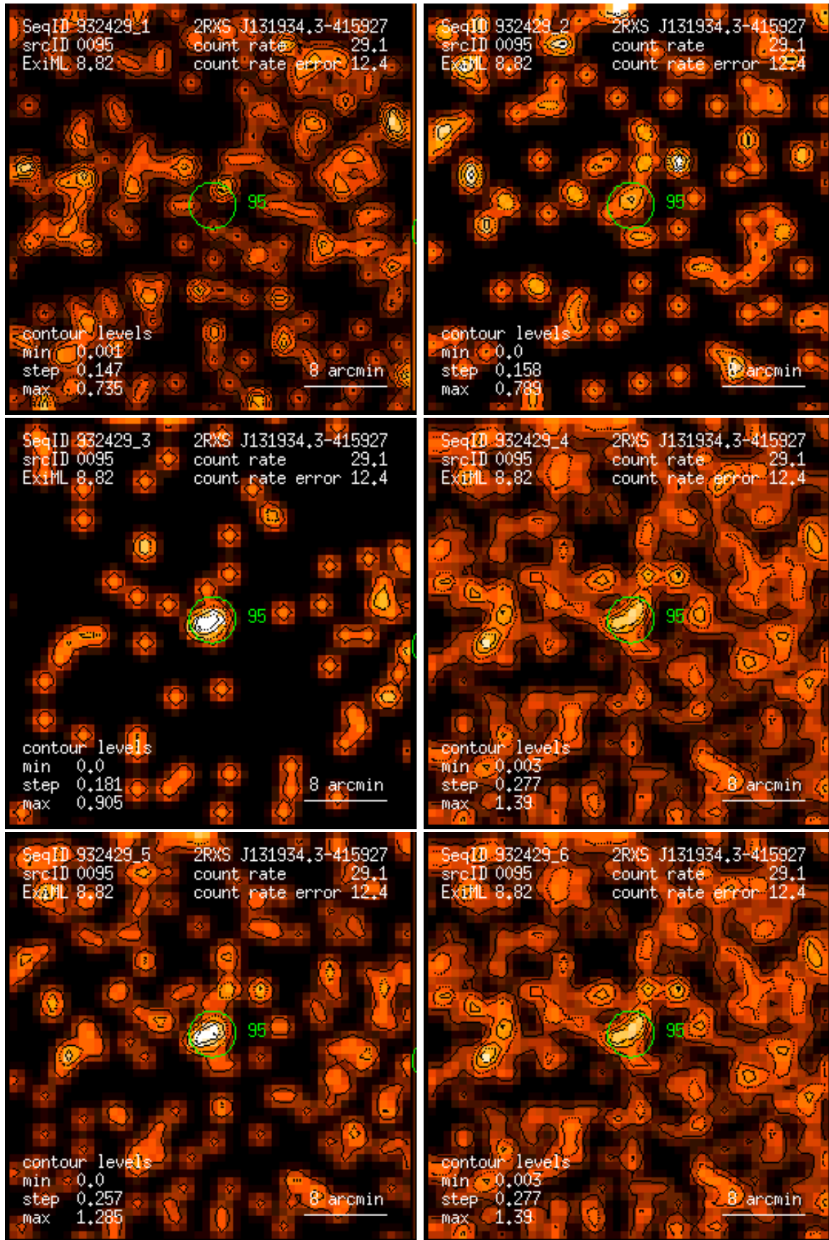
Figure 95: RASS 932429: detection 0095: band rate images, Gaussian filter: (1) PSPC channels 11 – 41, (2) 52 – 90, (3) 91 – 201, (4) 11 – 235, (5) 52 – 201, (6) 11 – 201. Broad band rates in counts/ks. Band rate contour levels in counts/ks/arcmin 2 .
