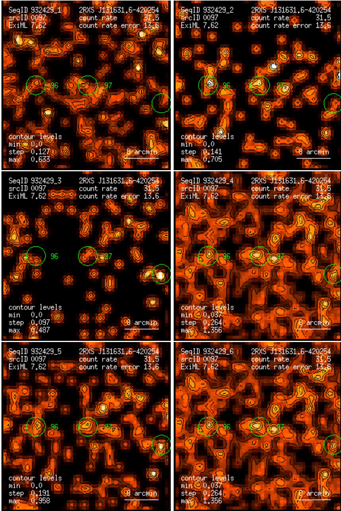
Figure 97: RASS 932429: detection 0097: band rate images, Gaussian filter: (1) PSPC channels 11 – 41, (2) 52 – 90, (3) 91 – 201, (4) 11 – 235, (5) 52 – 201, (6) 11 – 201. Broad band rates in counts/ks. Band rate contour levels in counts/ks/arcmin 2 .
