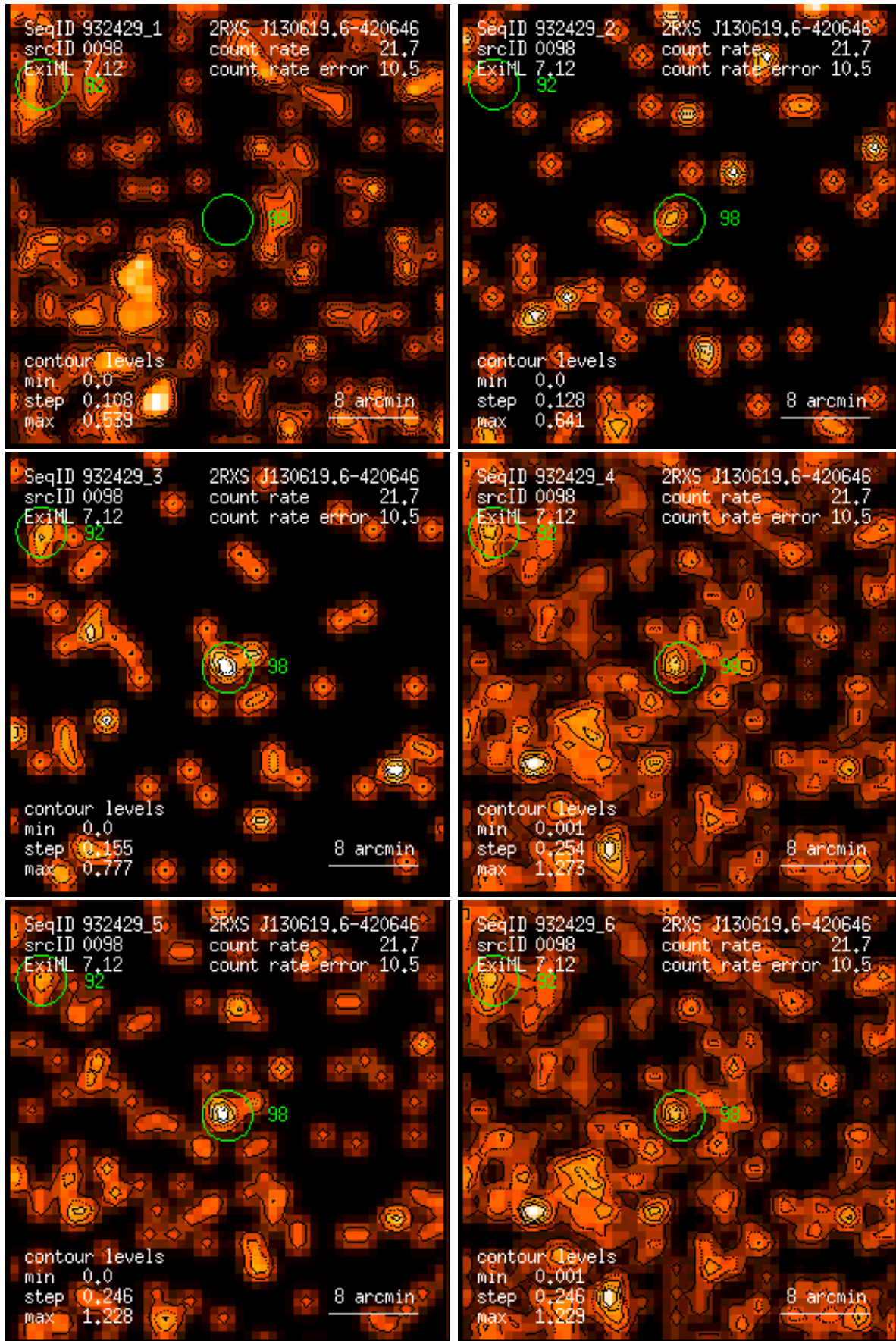
Figure 98: RASS 932429: detection 0098: band rate images, Gaussian filter: (1) PSPC channels 11 – 41, (2) 52 – 90, (3) 91 – 201, (4) 11 – 235, (5) 52 – 201, (6) 11 – 201. Broad band rates in counts/ks. Band rate contour levels in counts/ks/arcmin 2 .
