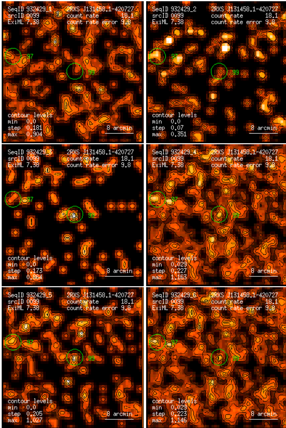
Figure 99: RASS 932429: detection 0099: band rate images, Gaussian filter: (1) PSPC channels 11 – 41, (2) 52 – 90, (3) 91 – 201, (4) 11 – 235, (5) 52 – 201, (6) 11 – 201. Broad band rates in counts/ks. Band rate contour levels in counts/ks/arcmin 2 .
