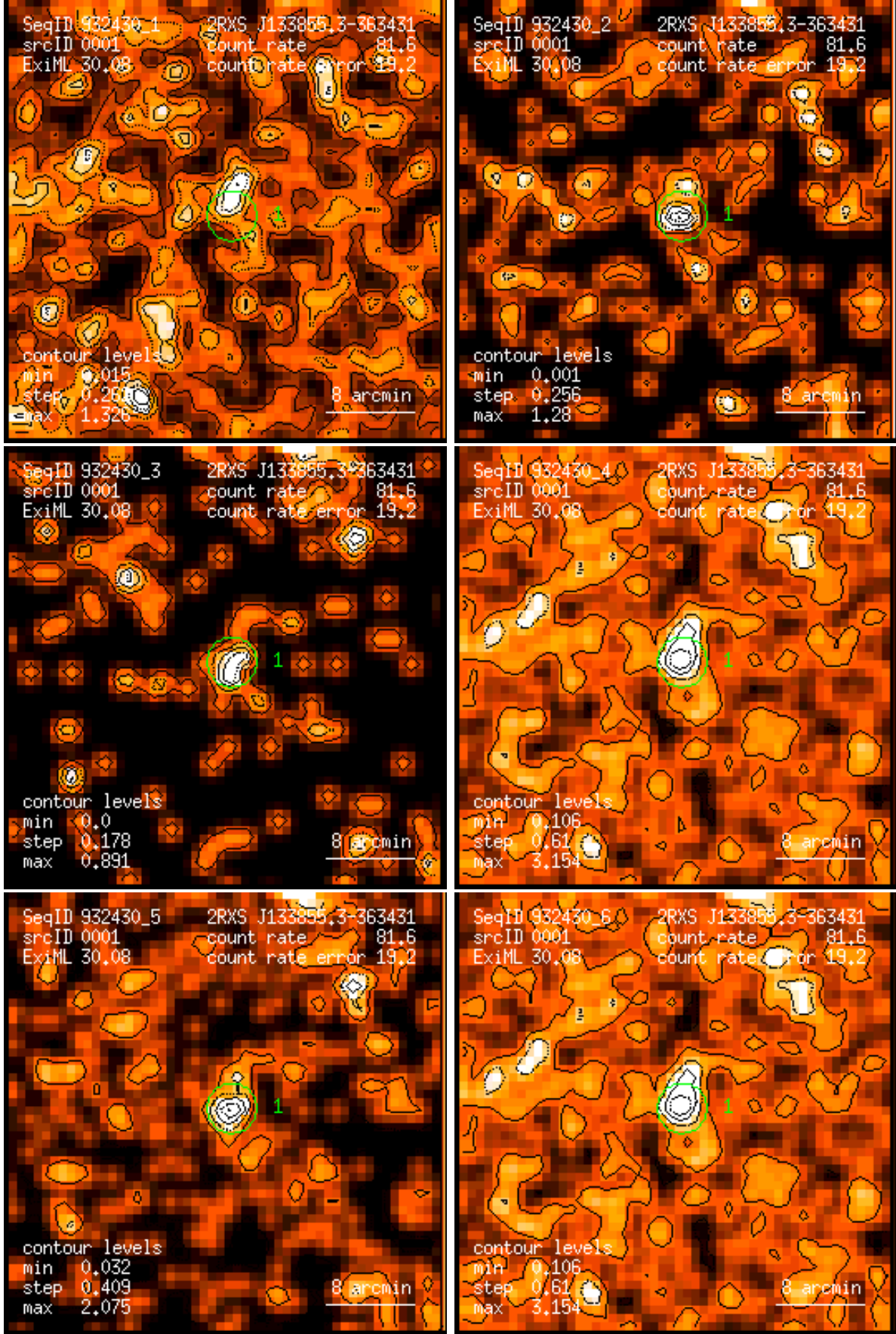
Figure 1: RASS 932430: detection 0001: band rate images, Gaussian filter: (1) PSPC channels 11 – 41, (2) 52 – 90, (3) 91 – 201, (4) 11 – 235, (5) 52 – 201, (6) 11 – 201. Broad band rates in counts/ks. Band rate contour levels in counts/ks/arcmin 2 .
