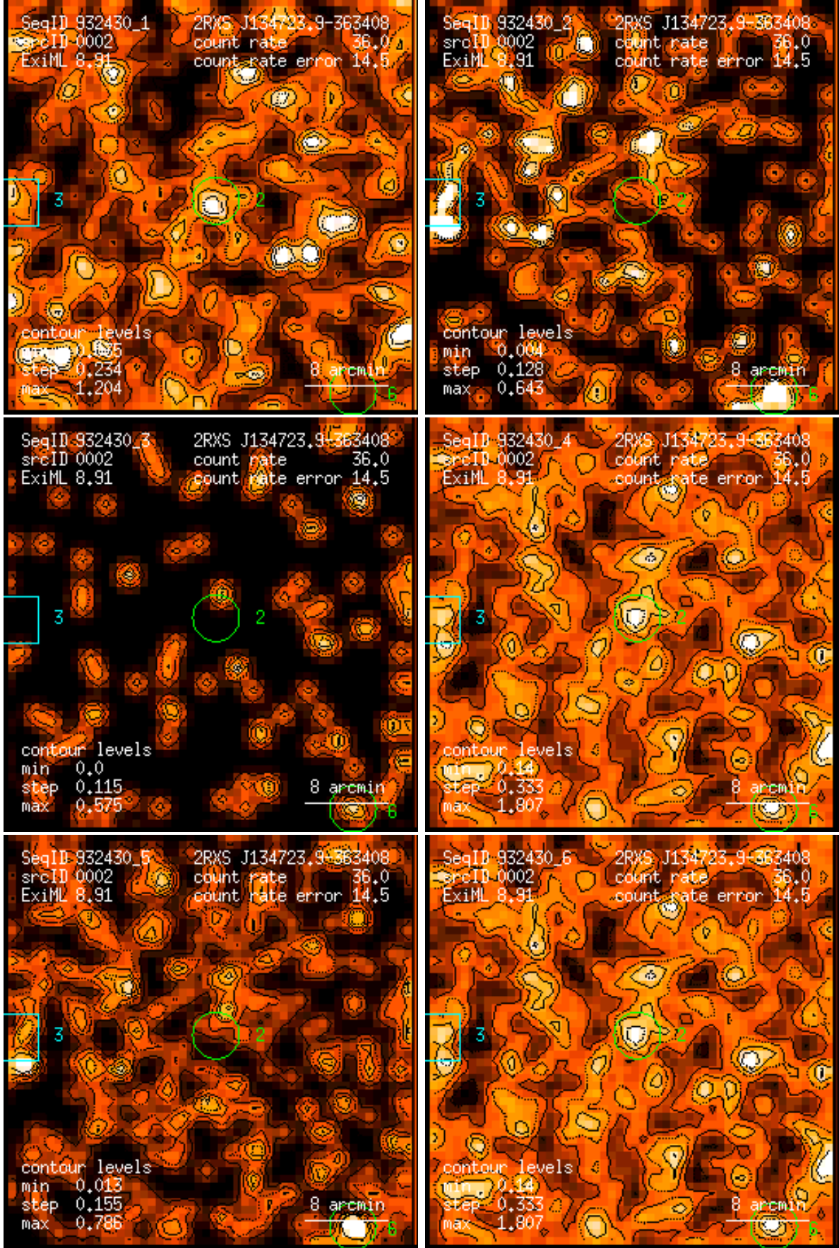
Figure 2: RASS 932430: detection 0002: band rate images, Gaussian filter: (1) PSPC channels 11 – 41, (2) 52 – 90, (3) 91 – 201, (4) 11 – 235, (5) 52 – 201, (6) 11 – 201. Broad band rates in counts/ks. Band rate contour levels in counts/ks/arcmin 2 .
