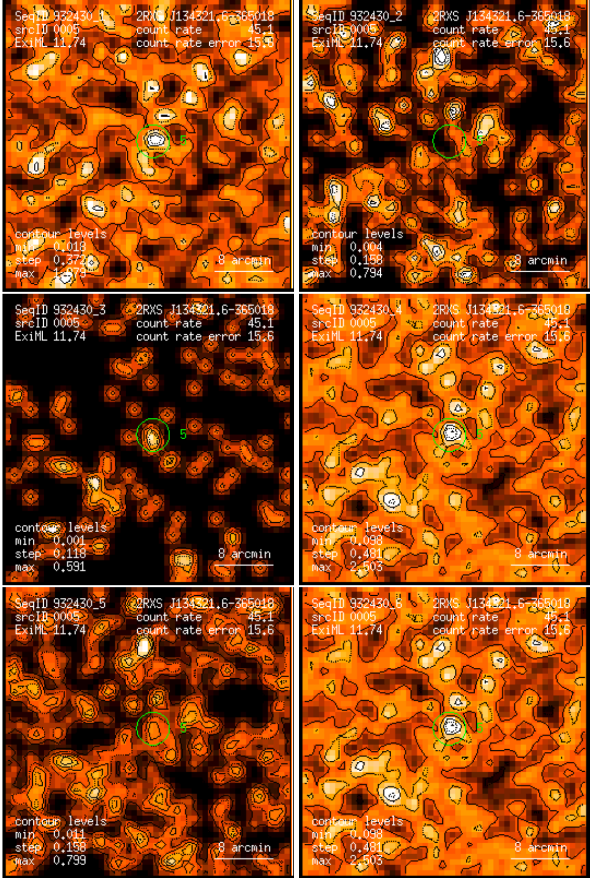
Figure 5: RASS 932430: detection 0005: band rate images, Gaussian filter: (1) PSPC channels 11 – 41, (2) 52 – 90, (3) 91 – 201, (4) 11 – 235, (5) 52 – 201, (6) 11 – 201. Broad band rates in counts/ks. Band rate contour levels in counts/ks/arcmin 2 .
