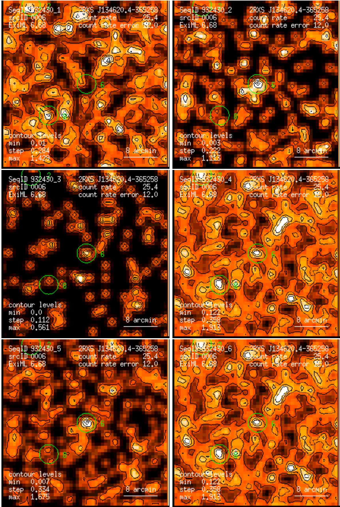
Figure 6: RASS 932430: detection 0006: band rate images, Gaussian filter: (1) PSPC channels 11 – 41, (2) 52 – 90, (3) 91 – 201, (4) 11 – 235, (5) 52 – 201, (6) 11 – 201. Broad band rates in counts/ks. Band rate contour levels in counts/ks/arcmin 2 .
