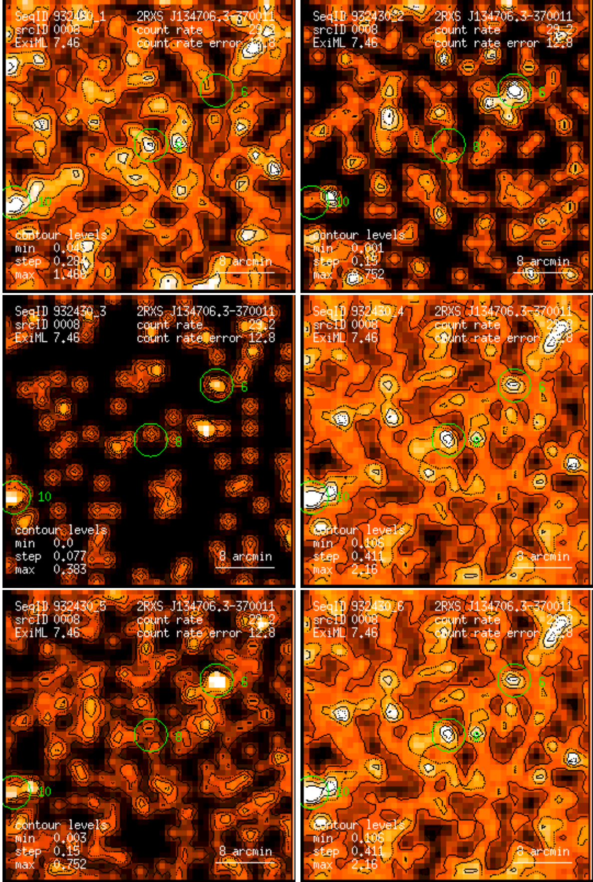
Figure 8: RASS 932430: detection 0008: band rate images, Gaussian filter: (1) PSPC channels 11 – 41, (2) 52 – 90, (3) 91 – 201, (4) 11 – 235, (5) 52 – 201, (6) 11 – 201. Broad band rates in counts/ks. Band rate contour levels in counts/ks/arcmin 2 .
