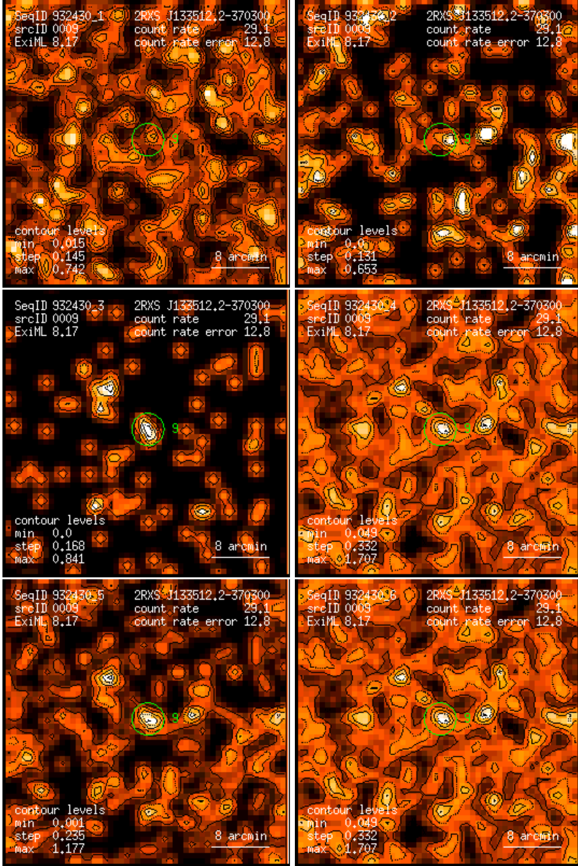
Figure 9: RASS 932430: detection 0009: band rate images, Gaussian filter: (1) PSPC channels 11 – 41, (2) 52 – 90, (3) 91 – 201, (4) 11 – 235, (5) 52 – 201, (6) 11 – 201. Broad band rates in counts/ks. Band rate contour levels in counts/ks/arcmin 2 .
