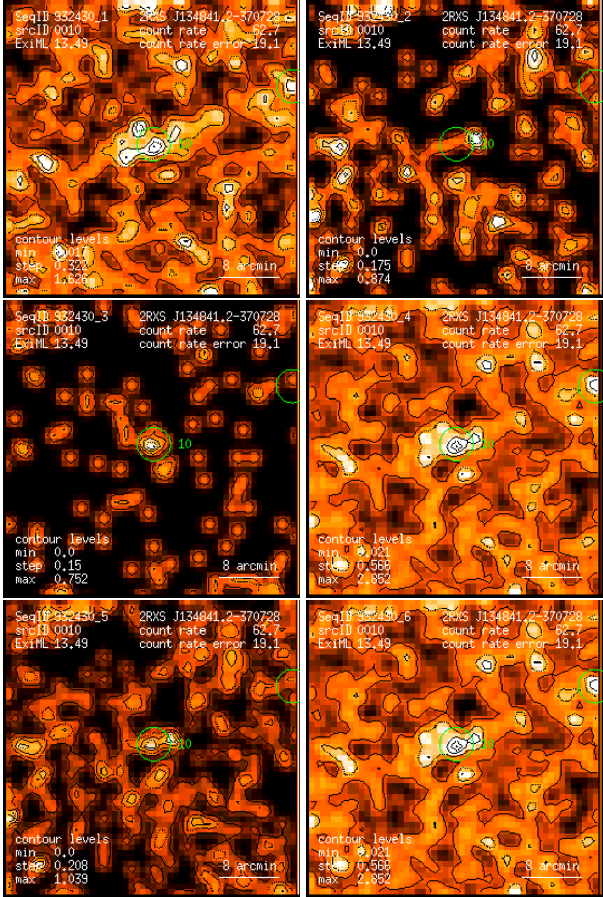
Figure 10: RASS 932430: detection 0010: band rate images, Gaussian filter: (1) PSPC channels 11 – 41, (2) 52 – 90, (3) 91 – 201, (4) 11 – 235, (5) 52 – 201, (6) 11 – 201. Broad band rates in counts/ks. Band rate contour levels in counts/ks/arcmin 2 .
