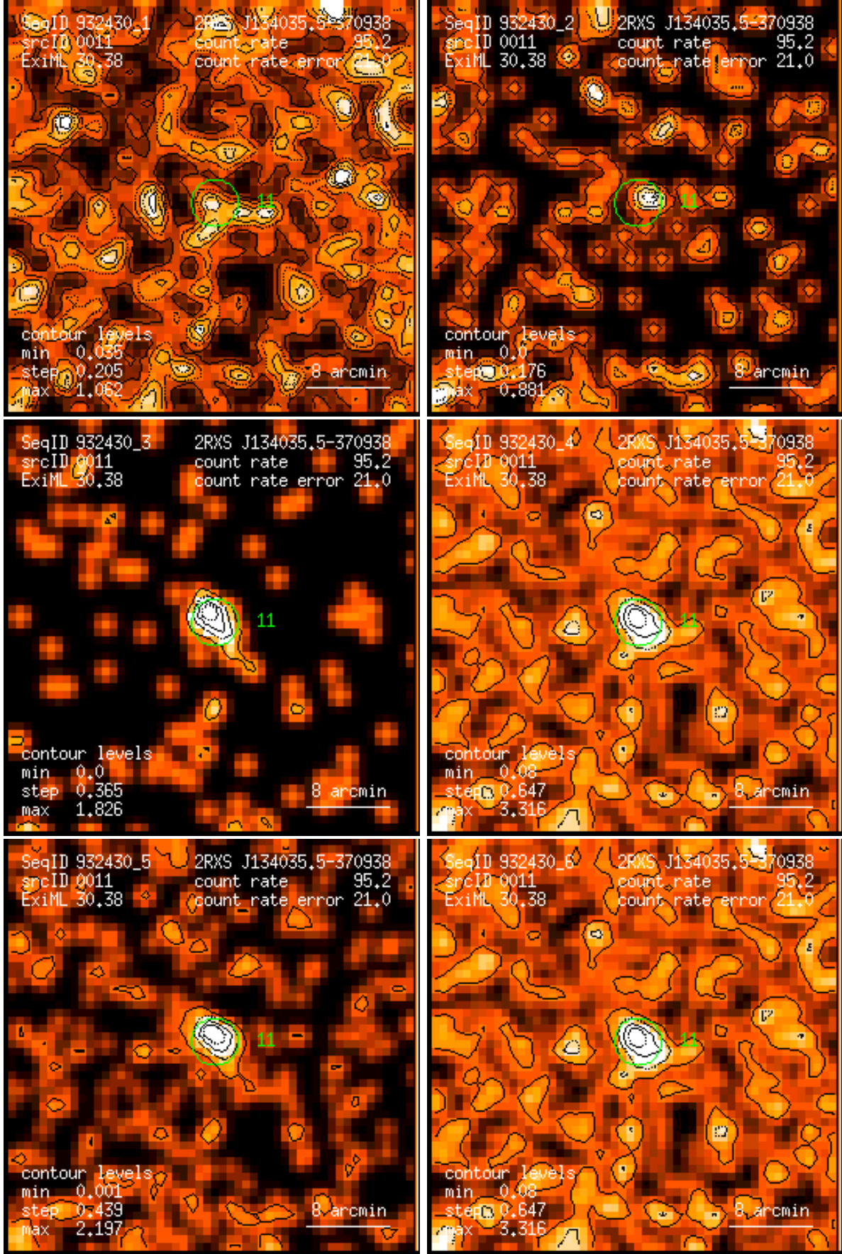
Figure 11: RASS 932430: detection 0011: band rate images, Gaussian filter: (1) PSPC channels 11 – 41, (2) 52 – 90, (3) 91 – 201, (4) 11 – 235, (5) 52 – 201, (6) 11 – 201. Broad band rates in counts/ks. Band rate contour levels in counts/ks/arcmin 2 .
