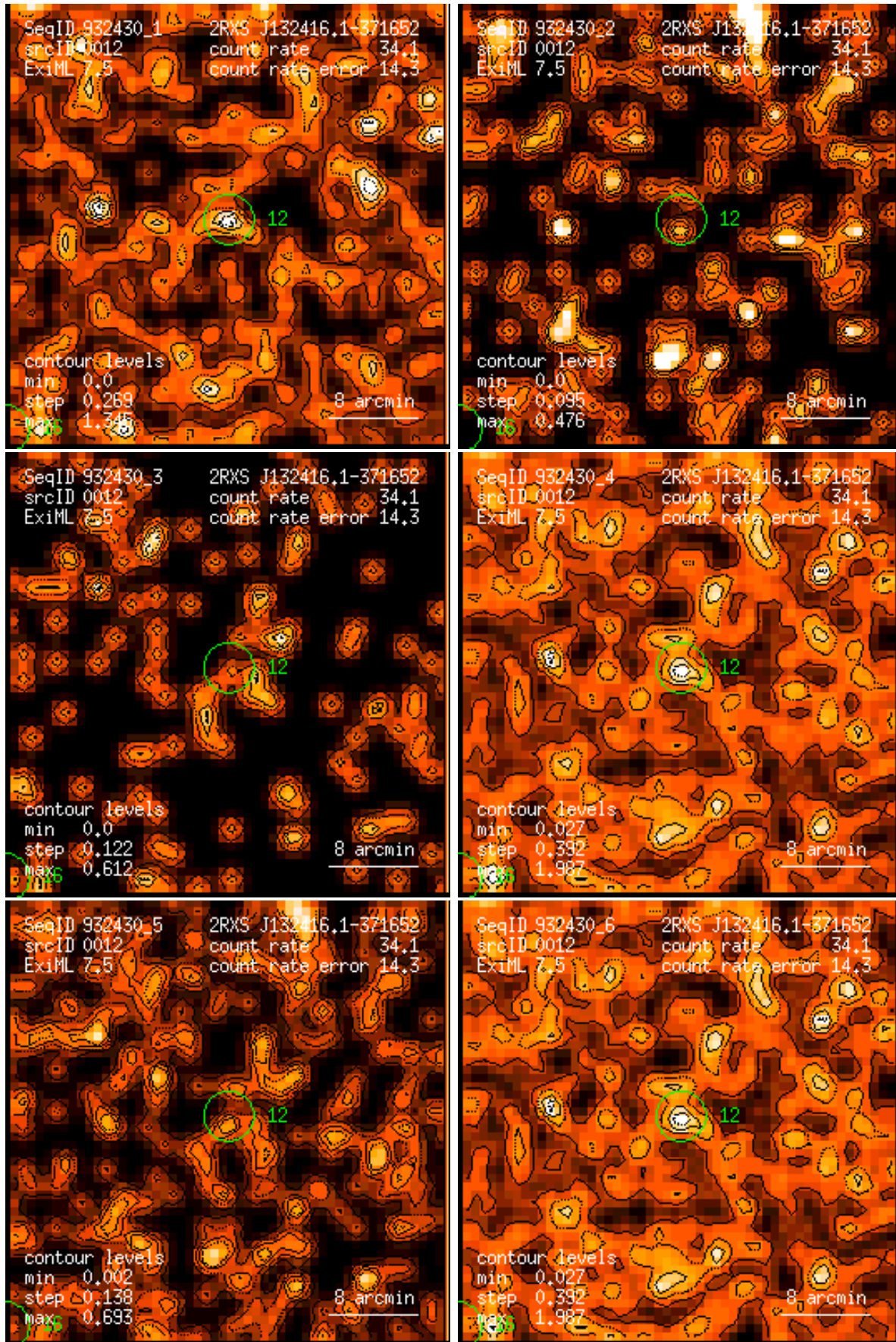
Figure 12: RASS 932430: detection 0012: band rate images, Gaussian filter: (1) PSPC channels 11 – 41, (2) 52 – 90, (3) 91 – 201, (4) 11 – 235, (5) 52 – 201, (6) 11 – 201. Broad band rates in counts/ks. Band rate contour levels in counts/ks/arcmin 2 .
