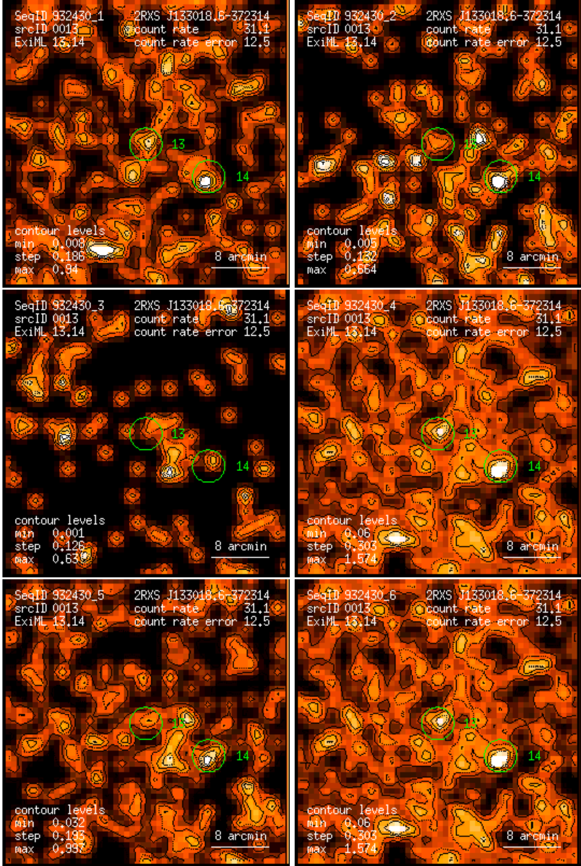
Figure 13: RASS 932430: detection 0013: band rate images, Gaussian filter: (1) PSPC channels 11 – 41, (2) 52 – 90, (3) 91 – 201, (4) 11 – 235, (5) 52 – 201, (6) 11 – 201. Broad band rates in counts/ks. Band rate contour levels in counts/ks/arcmin 2 .
